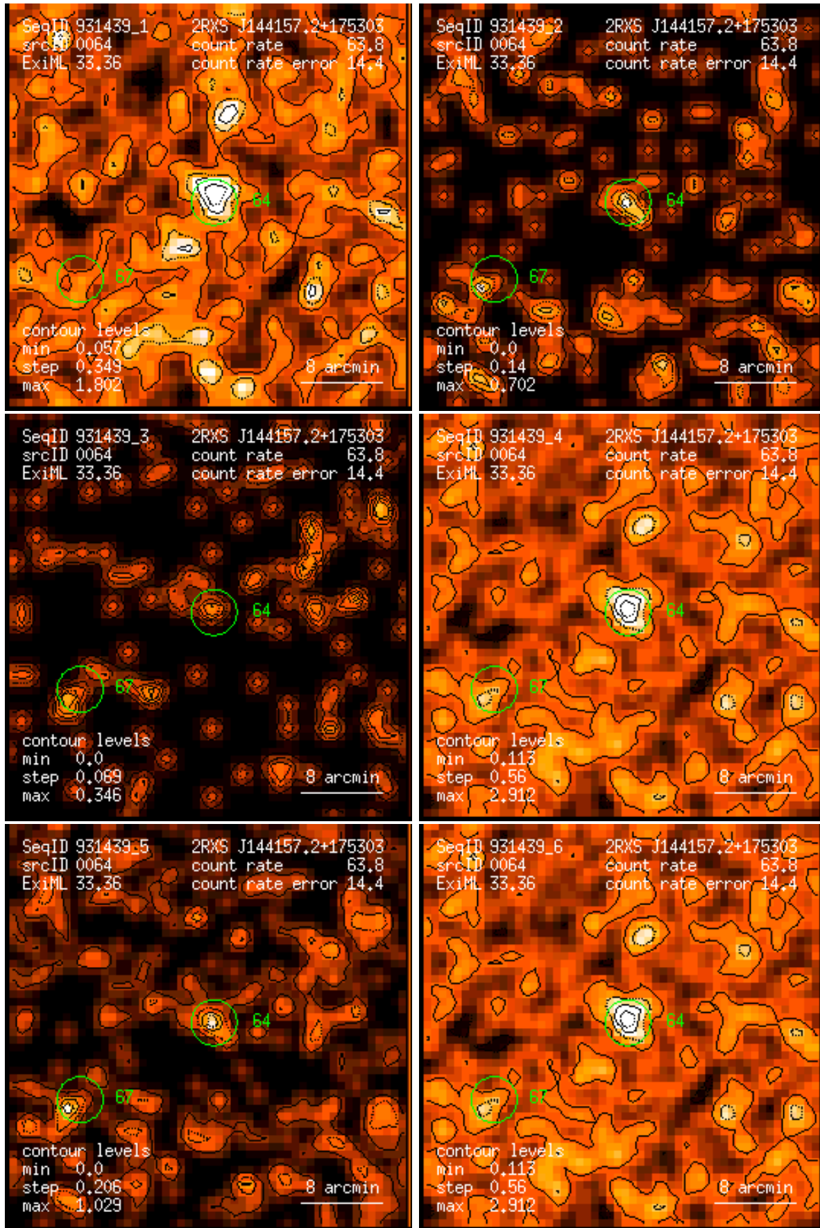
Figure 64: RASS 931439: detection 0064: band rate images, Gaussian filter: (1) PSPC channels 11 – 41, (2) 52 – 90, (3) 91 – 201, (4) 11 – 235, (5) 52 – 201, (6) 11 – 201. Broad band rates in counts/ks. Band rate contour levels in counts/ks/arcmin 2 .
