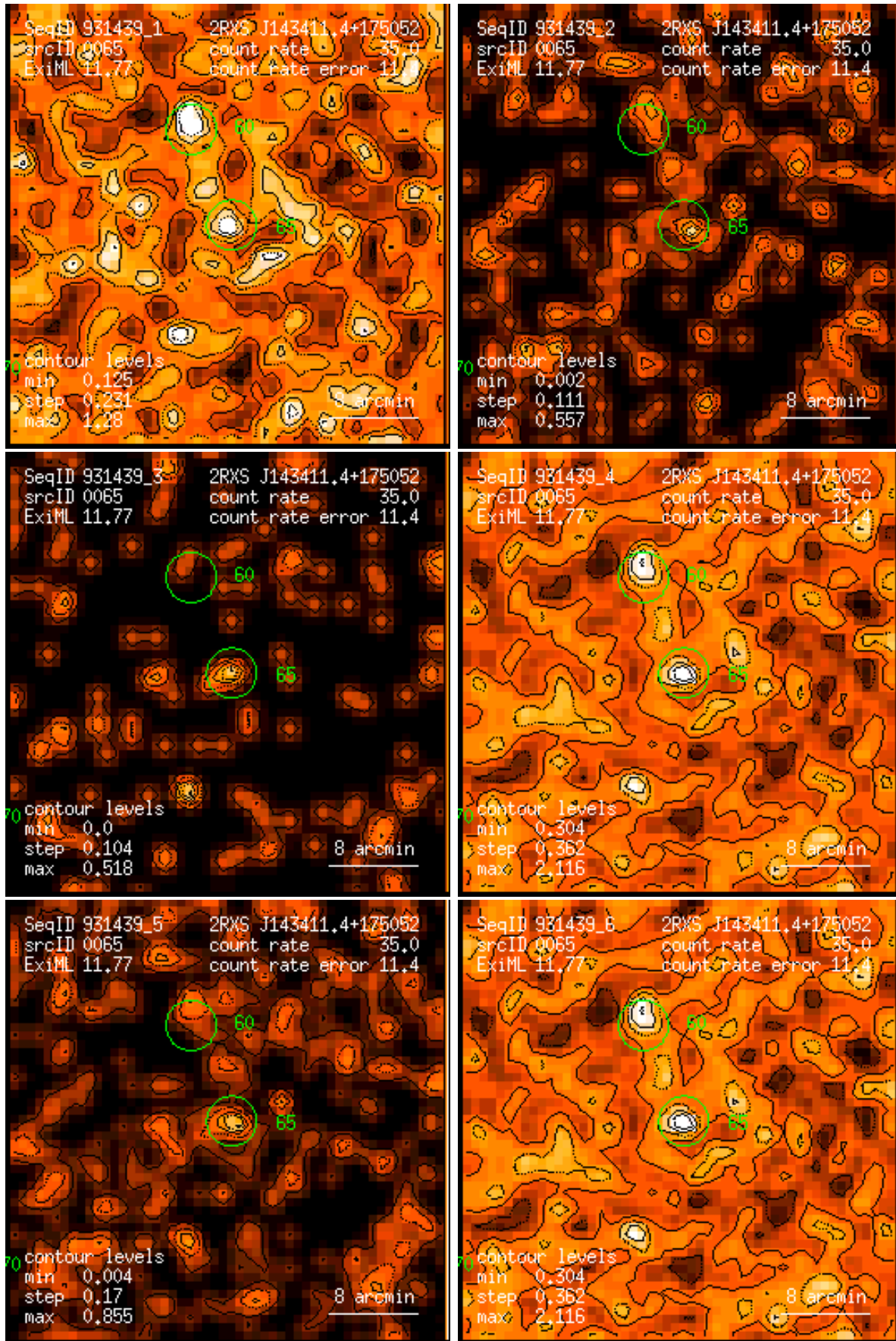
Figure 65: RASS 931439: detection 0065: band rate images, Gaussian filter: (1) PSPC channels 11 – 41, (2) 52 – 90, (3) 91 – 201, (4) 11 – 235, (5) 52 – 201, (6) 11 – 201. Broad band rates in counts/ks. Band rate contour levels in counts/ks/arcmin 2 .
