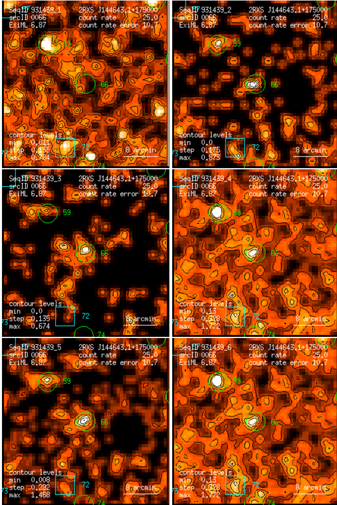
Figure 66: RASS 931439: detection 0066: band rate images, Gaussian filter: (1) PSPC channels 11 – 41, (2) 52 – 90, (3) 91 – 201, (4) 11 – 235, (5) 52 – 201, (6) 11 – 201. Broad band rates in counts/ks. Band rate contour levels in counts/ks/arcmin 2 .
