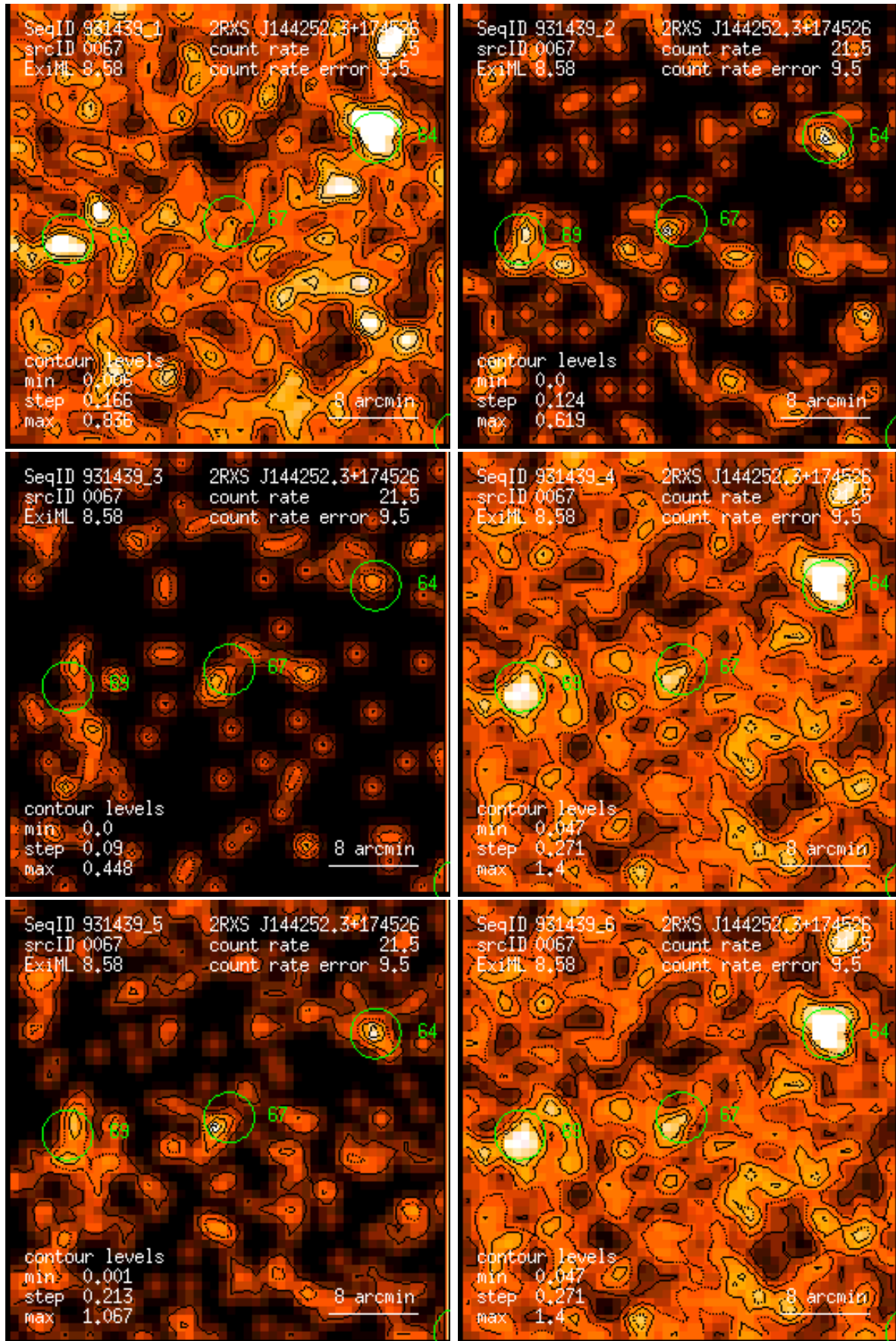
Figure 67: RASS 931439: detection 0067: band rate images, Gaussian filter: (1) PSPC channels 11 – 41, (2) 52 – 90, (3) 91 – 201, (4) 11 – 235, (5) 52 – 201, (6) 11 – 201. Broad band rates in counts/ks. Band rate contour levels in counts/ks/arcmin 2 .
