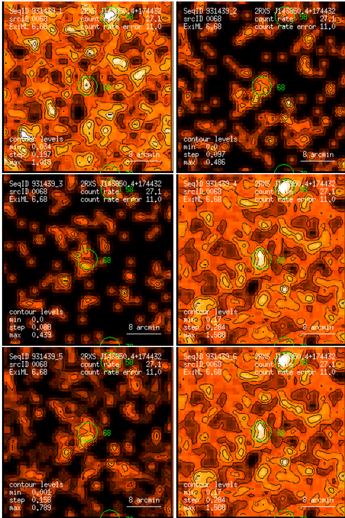
Figure 68: RASS 931439: detection 0068: band rate images, Gaussian filter: (1) PSPC channels 11 – 41, (2) 52 – 90, (3) 91 – 201, (4) 11 – 235, (5) 52 – 201, (6) 11 – 201. Broad band rates in counts/ks. Band rate contour levels in counts/ks/arcmin 2 .
