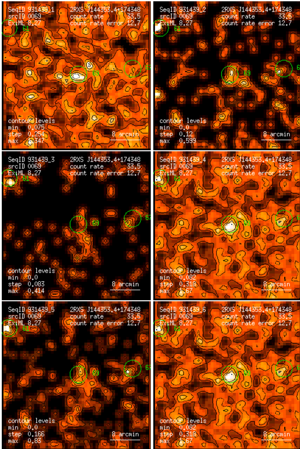
Figure 69: RASS 931439: detection 0069: band rate images, Gaussian filter: (1) PSPC channels 11 – 41, (2) 52 – 90, (3) 91 – 201, (4) 11 – 235, (5) 52 – 201, (6) 11 – 201. Broad band rates in counts/ks. Band rate contour levels in counts/ks/arcmin 2 .
