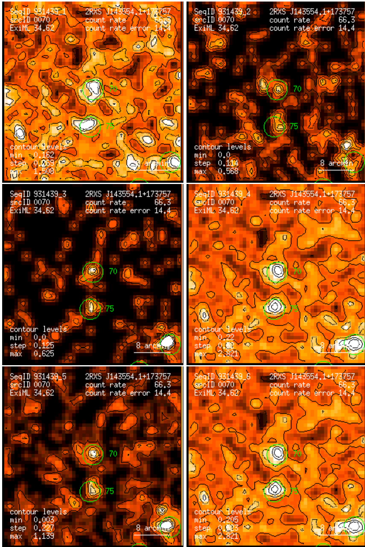
Figure 70: RASS 931439: detection 0070: band rate images, Gaussian filter: (1) PSPC channels 11 – 41, (2) 52 – 90, (3) 91 – 201, (4) 11 – 235, (5) 52 – 201, (6) 11 – 201. Broad band rates in counts/ks. Band rate contour levels in counts/ks/arcmin 2 .
