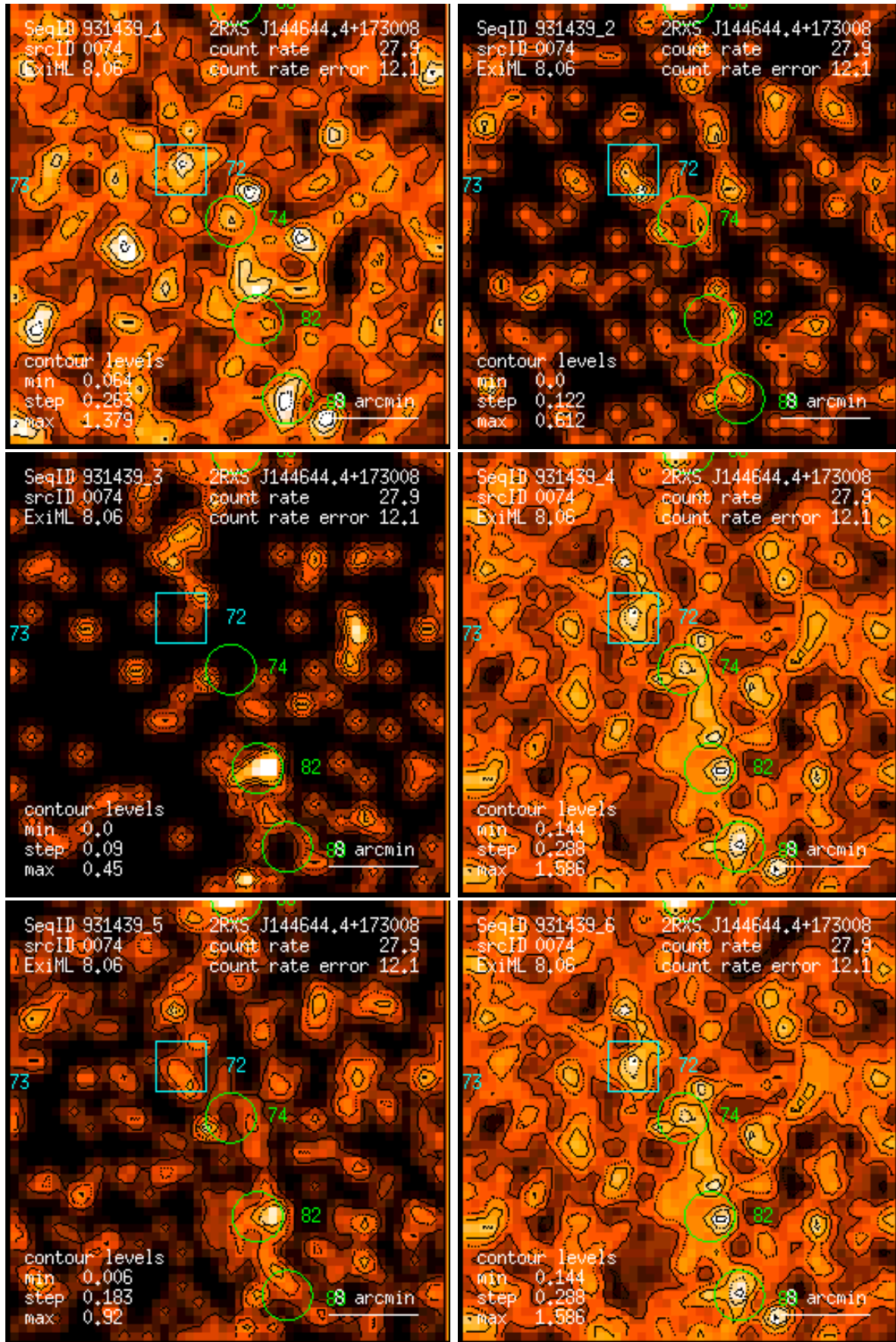
Figure 74: RASS 931439: detection 0074: band rate images, Gaussian filter: (1) PSPC channels 11 – 41, (2) 52 – 90, (3) 91 – 201, (4) 11 – 235, (5) 52 – 201, (6) 11 – 201. Broad band rates in counts/ks. Band rate contour levels in counts/ks/arcmin 2 .
