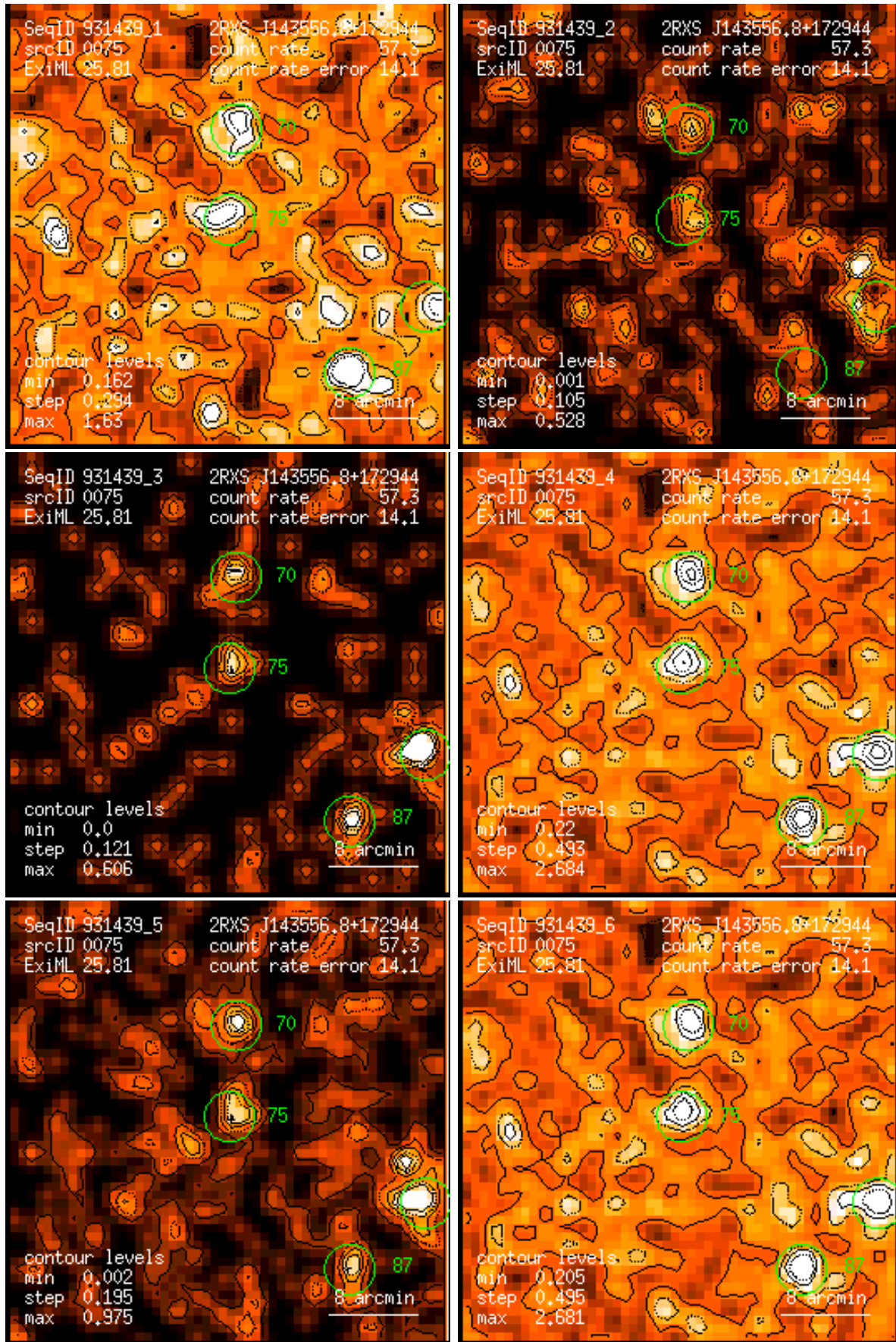
Figure 75: RASS 931439: detection 0075: band rate images, Gaussian filter: (1) PSPC channels 11 – 41, (2) 52 – 90, (3) 91 – 201, (4) 11 – 235, (5) 52 – 201, (6) 11 – 201. Broad band rates in counts/ks. Band rate contour levels in counts/ks/arcmin 2 .
