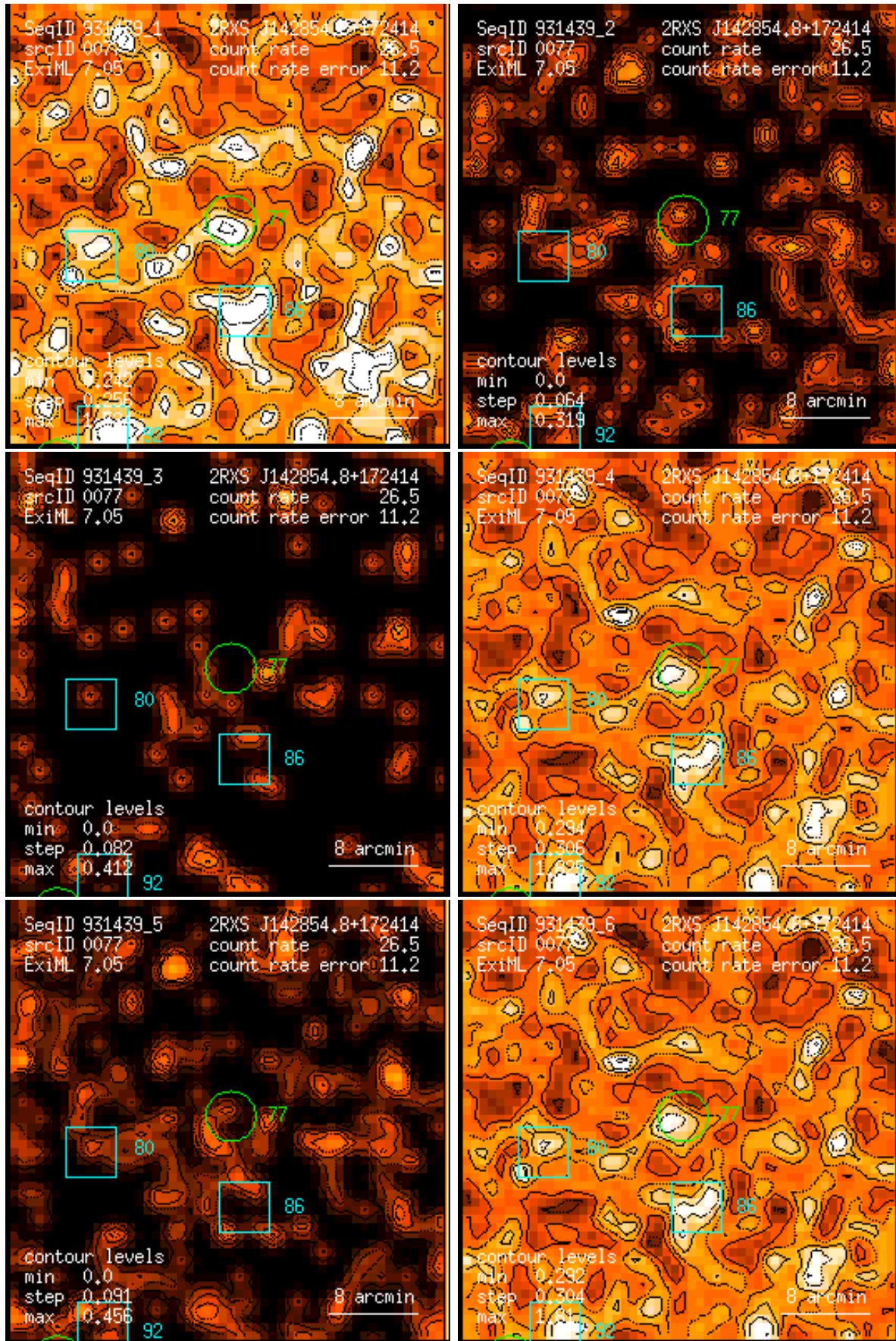
Figure 77: RASS 931439: detection 0077: band rate images, Gaussian filter: (1) PSPC channels 11 – 41, (2) 52 – 90, (3) 91 – 201, (4) 11 – 235, (5) 52 – 201, (6) 11 – 201. Broad band rates in counts/ks. Band rate contour levels in counts/ks/arcmin 2 .
