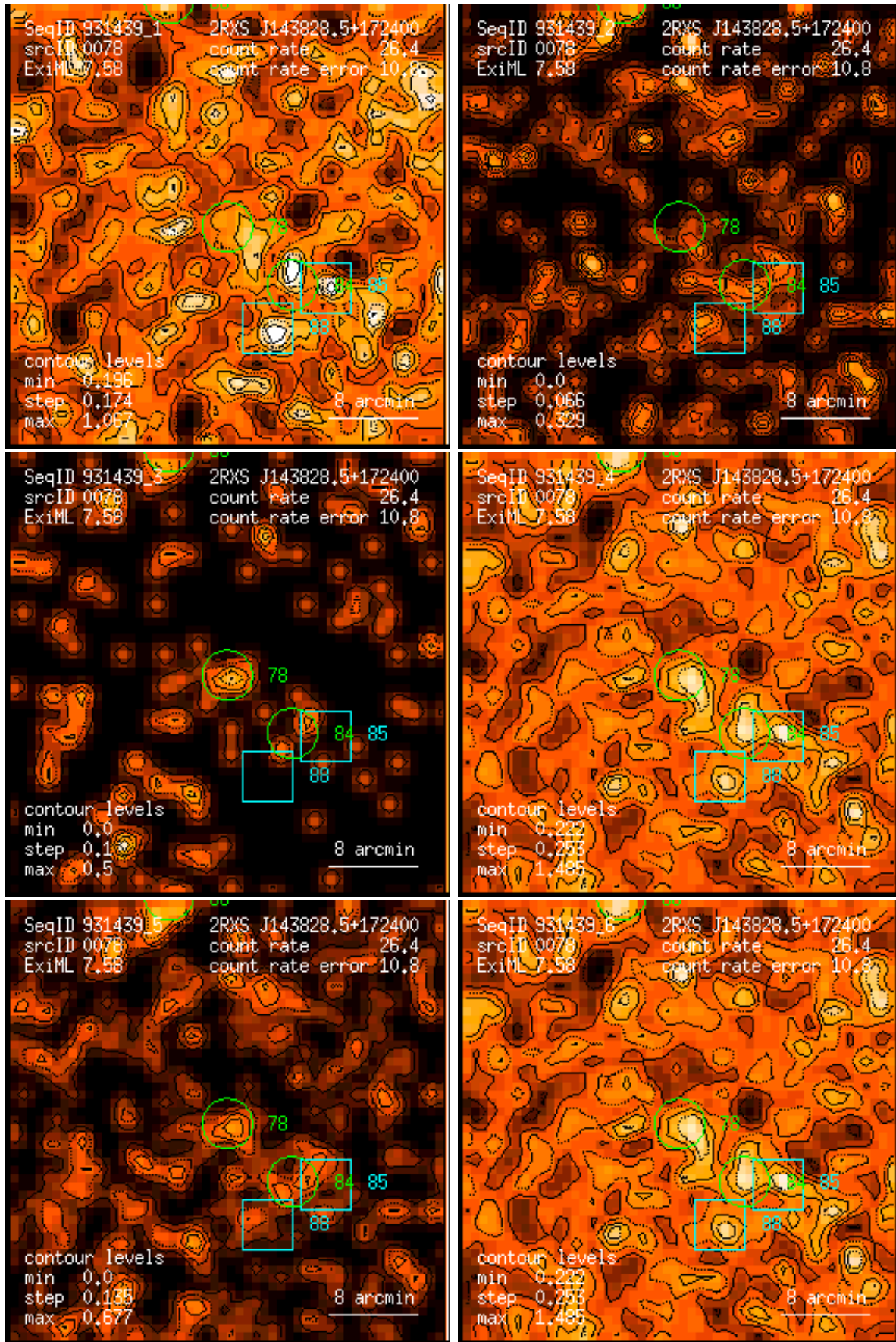
Figure 78: RASS 931439: detection 0078: band rate images, Gaussian filter: (1) PSPC channels 11 – 41, (2) 52 – 90, (3) 91 – 201, (4) 11 – 235, (5) 52 – 201, (6) 11 – 201. Broad band rates in counts/ks. Band rate contour levels in counts/ks/arcmin 2 .
