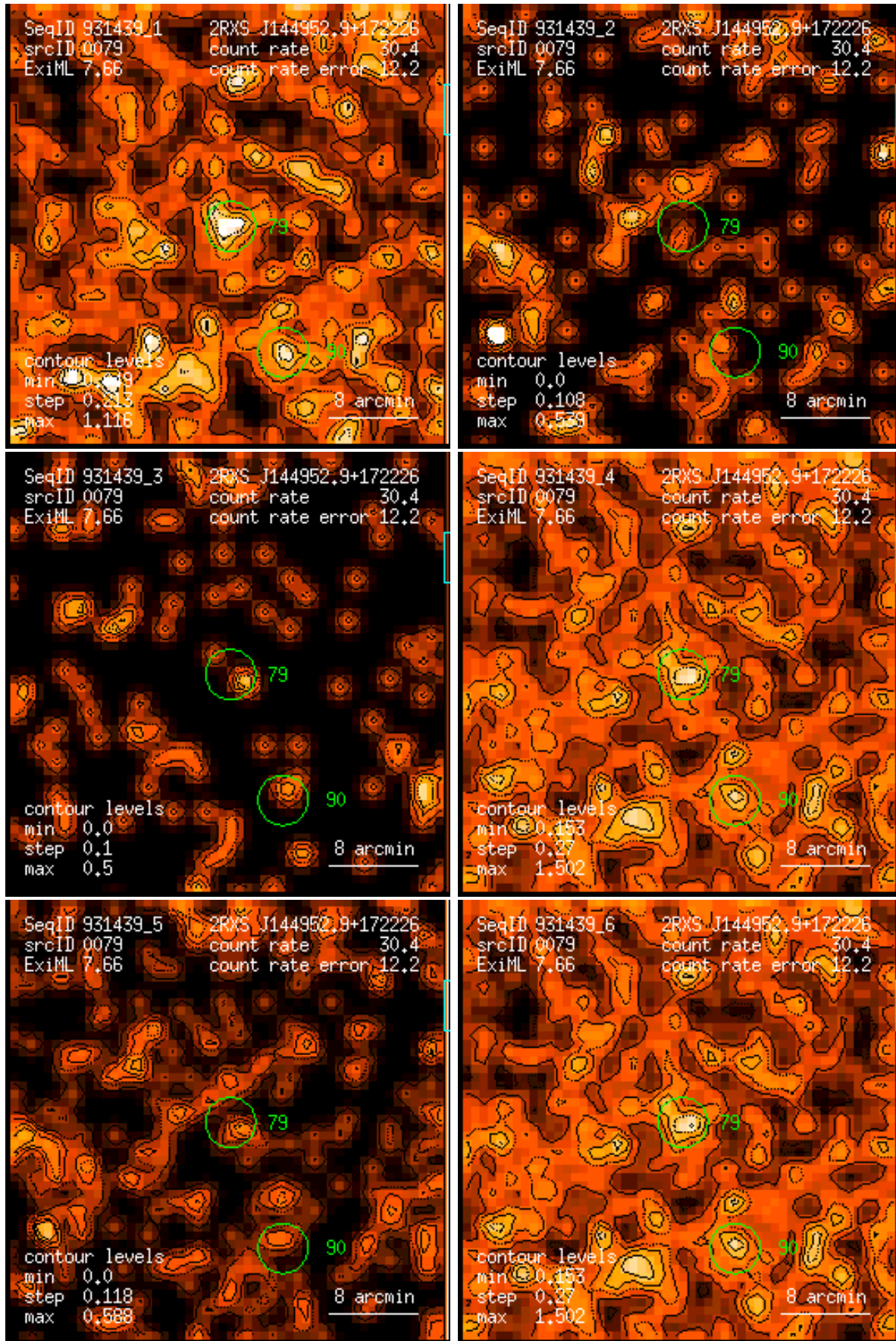
Figure 79: RASS 931439: detection 0079: band rate images, Gaussian filter: (1) PSPC channels 11 – 41, (2) 52 – 90, (3) 91 – 201, (4) 11 – 235, (5) 52 – 201, (6) 11 – 201. Broad band rates in counts/ks. Band rate contour levels in counts/ks/arcmin 2 .
