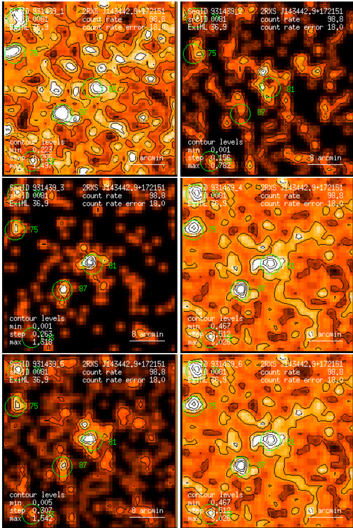
Figure 81: RASS 931439: detection 0081: band rate images, Gaussian filter: (1) PSPC channels 11 – 41, (2) 52 – 90, (3) 91 – 201, (4) 11 – 235, (5) 52 – 201, (6) 11 – 201. Broad band rates in counts/ks. Band rate contour levels in counts/ks/arcmin 2 .
