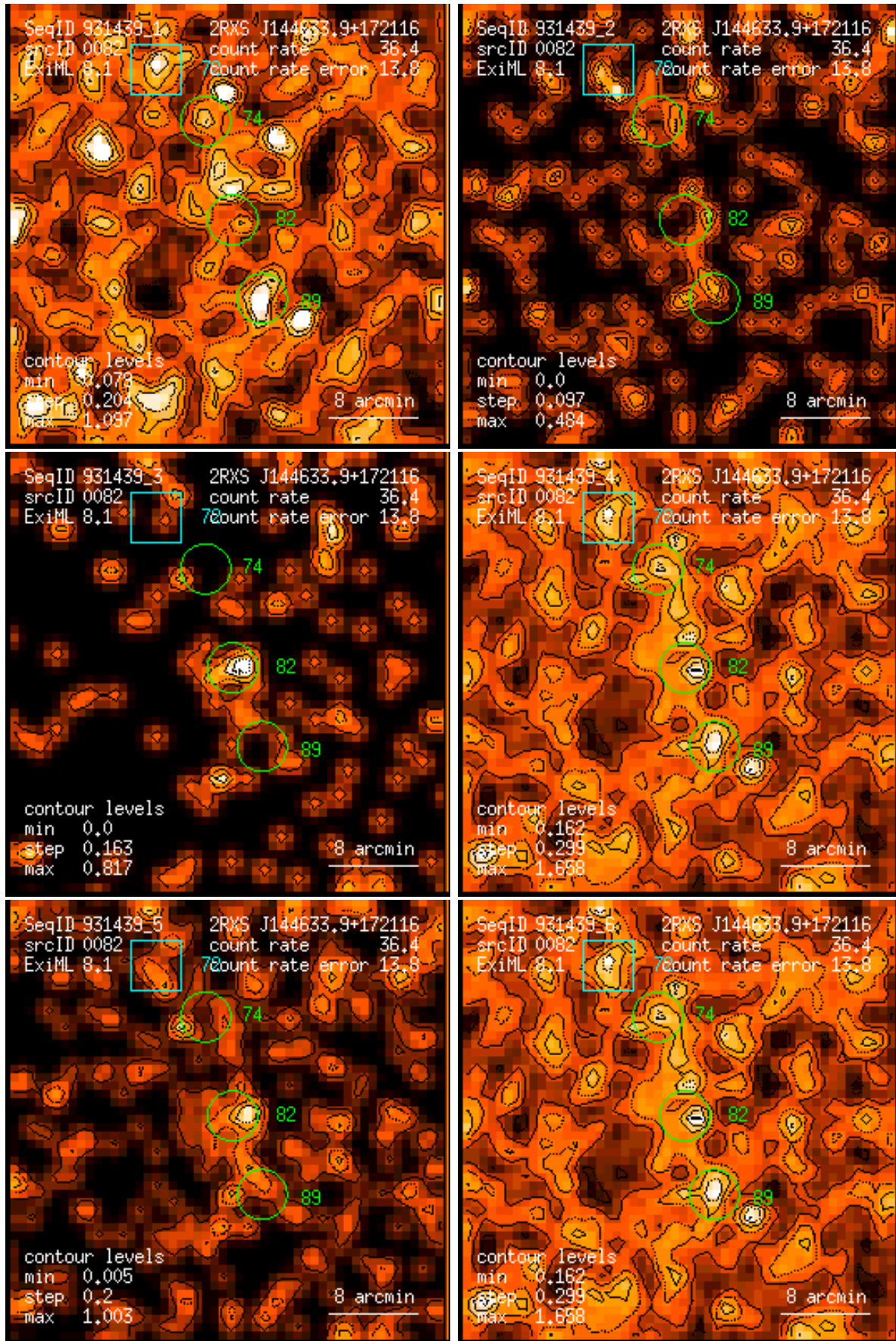
Figure 82: RASS 931439: detection 0082: band rate images, Gaussian filter: (1) PSPC channels 11 – 41, (2) 52 – 90, (3) 91 – 201, (4) 11 – 235, (5) 52 – 201, (6) 11 – 201. Broad band rates in counts/ks. Band rate contour levels in counts/ks/arcmin 2 .
