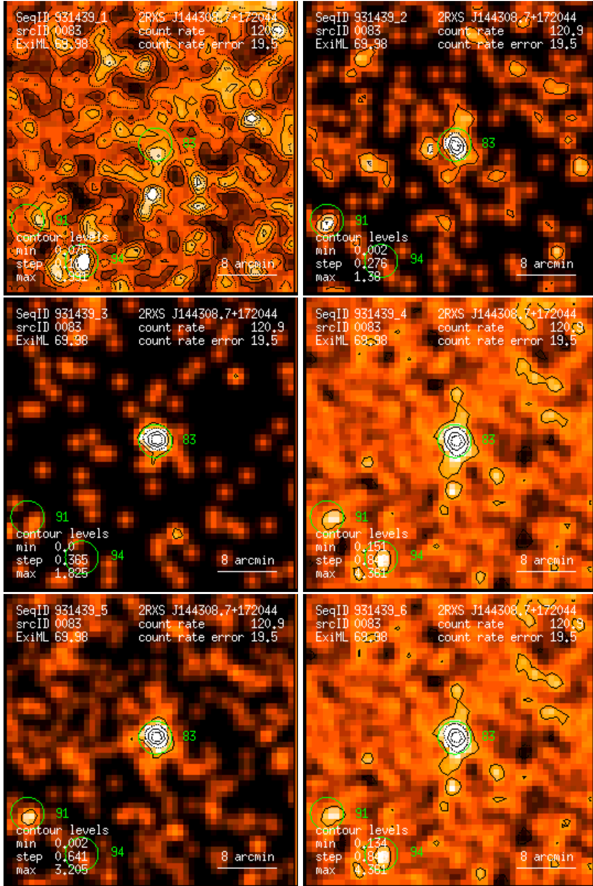
Figure 83: RASS 931439: detection 0083: band rate images, Gaussian filter: (1) PSPC channels 11 – 41, (2) 52 – 90, (3) 91 – 201, (4) 11 – 235, (5) 52 – 201, (6) 11 – 201. Broad band rates in counts/ks. Band rate contour levels in counts/ks/arcmin 2 .
