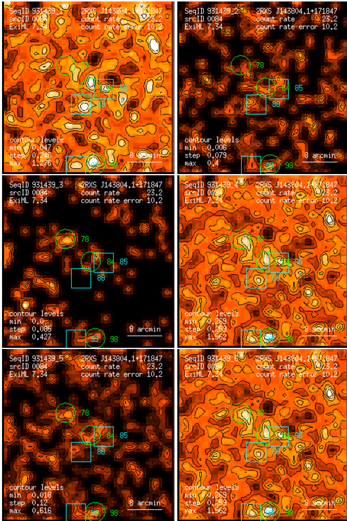
Figure 84: RASS 931439: detection 0084: band rate images, Gaussian filter: (1) PSPC channels 11 – 41, (2) 52 – 90, (3) 91 – 201, (4) 11 – 235, (5) 52 – 201, (6) 11 – 201. Broad band rates in counts/ks. Band rate contour levels in counts/ks/arcmin 2 .
