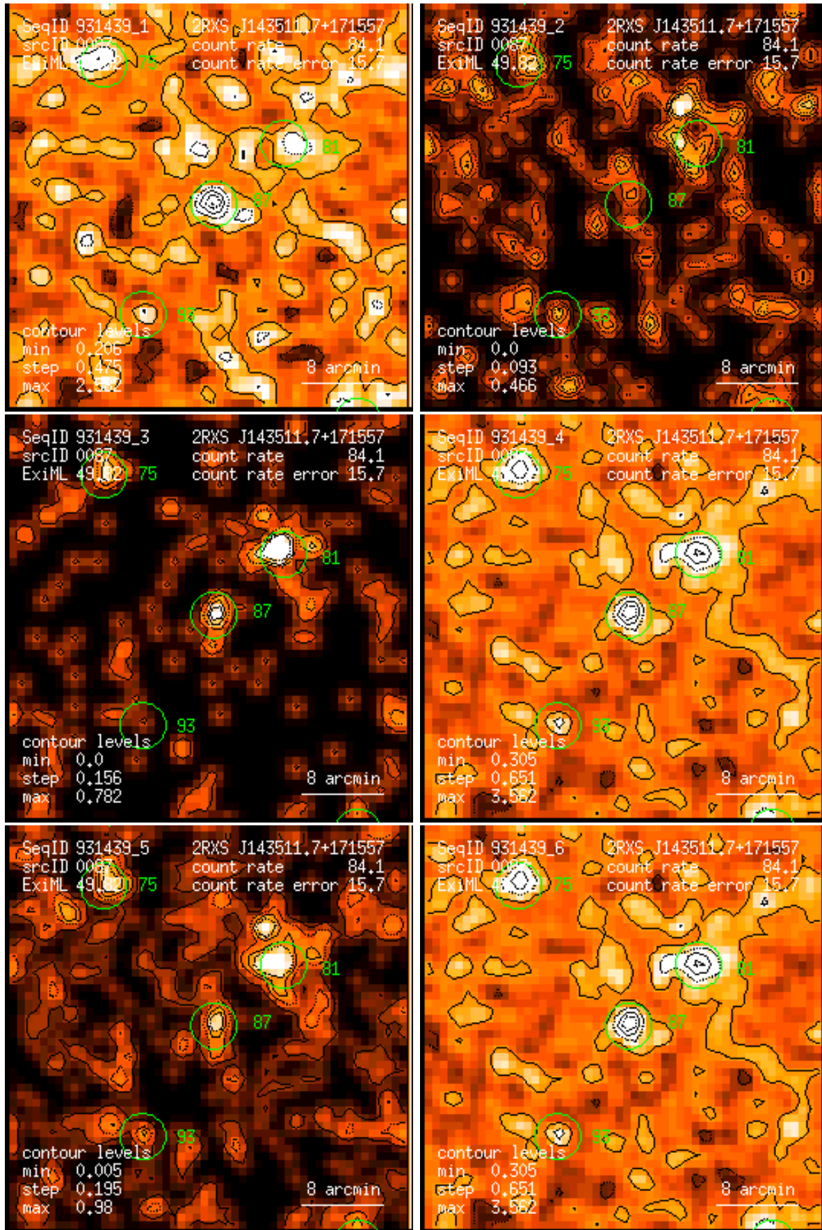
Figure 87: RASS 931439: detection 0087: band rate images, Gaussian filter: (1) PSPC channels 11 – 41, (2) 52 – 90, (3) 91 – 201, (4) 11 – 235, (5) 52 – 201, (6) 11 – 201. Broad band rates in counts/ks. Band rate contour levels in counts/ks/arcmin 2 .
