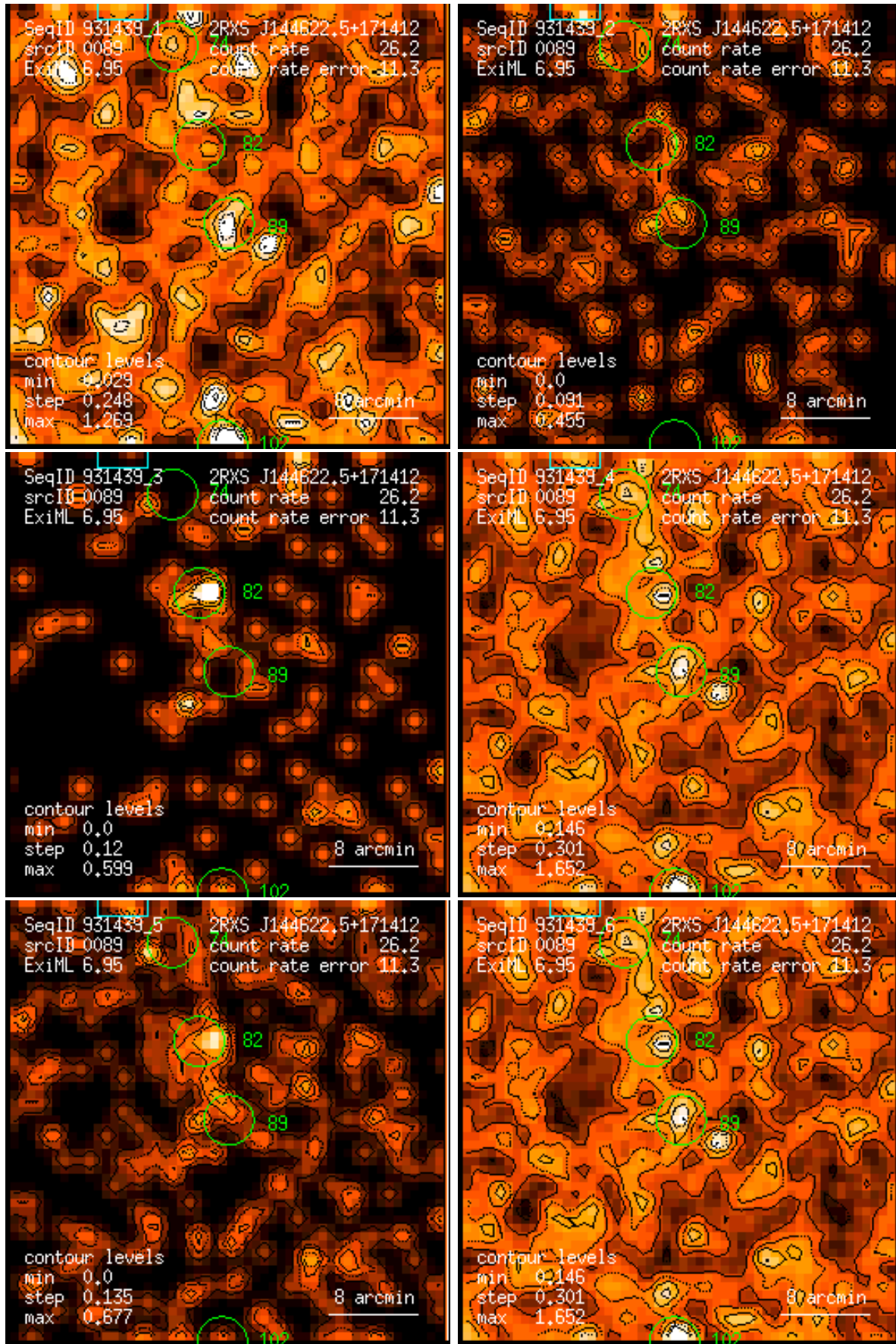
Figure 89: RASS 931439: detection 0089: band rate images, Gaussian filter: (1) PSPC channels 11 – 41, (2) 52 – 90, (3) 91 – 201, (4) 11 – 235, (5) 52 – 201, (6) 11 – 201. Broad band rates in counts/ks. Band rate contour levels in counts/ks/arcmin 2 .
