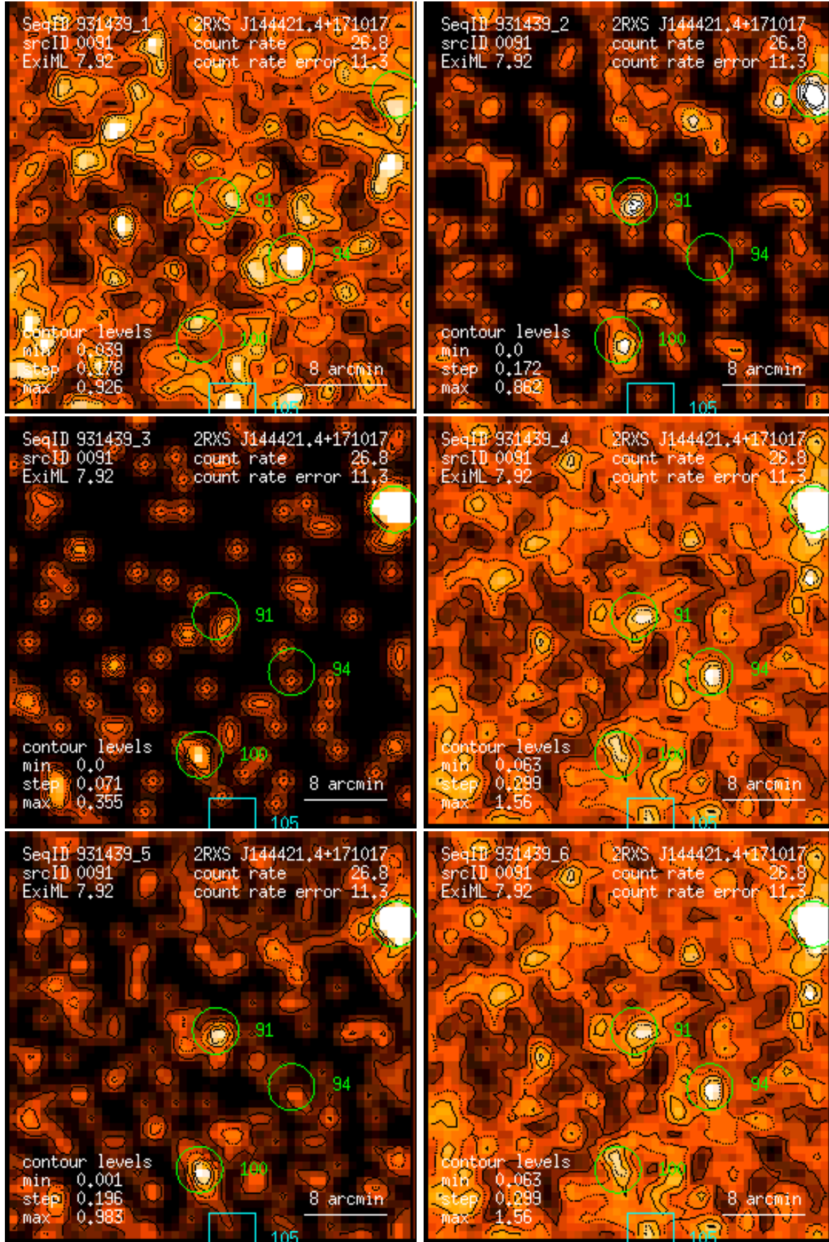
Figure 91: RASS 931439: detection 0091: band rate images, Gaussian filter: (1) PSPC channels 11 – 41, (2) 52 – 90, (3) 91 – 201, (4) 11 – 235, (5) 52 – 201, (6) 11 – 201. Broad band rates in counts/ks. Band rate contour levels in counts/ks/arcmin 2 .
