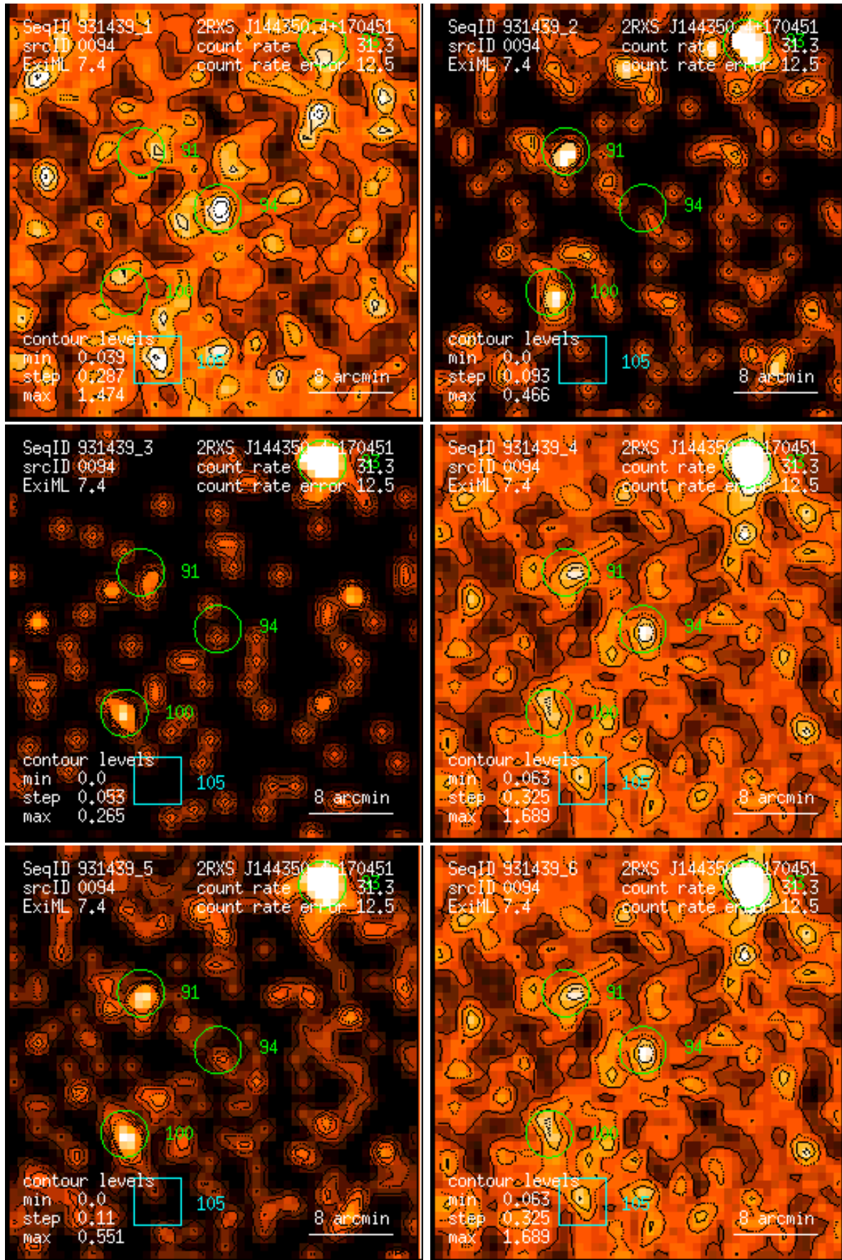
Figure 94: RASS 931439: detection 0094: band rate images, Gaussian filter: (1) PSPC channels 11 – 41, (2) 52 – 90, (3) 91 – 201, (4) 11 – 235, (5) 52 – 201, (6) 11 – 201. Broad band rates in counts/ks. Band rate contour levels in counts/ks/arcmin 2 .
