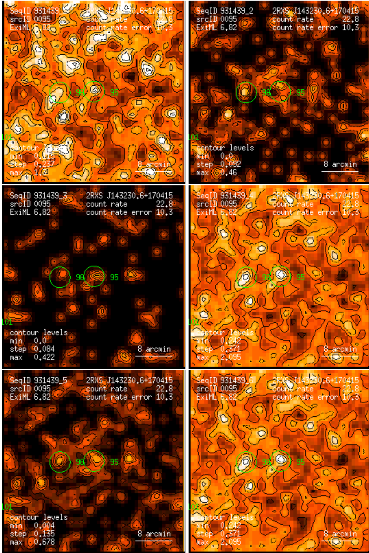
Figure 95: RASS 931439: detection 0095: band rate images, Gaussian filter: (1) PSPC channels 11 – 41, (2) 52 – 90, (3) 91 – 201, (4) 11 – 235, (5) 52 – 201, (6) 11 – 201. Broad band rates in counts/ks. Band rate contour levels in counts/ks/arcmin 2 .
