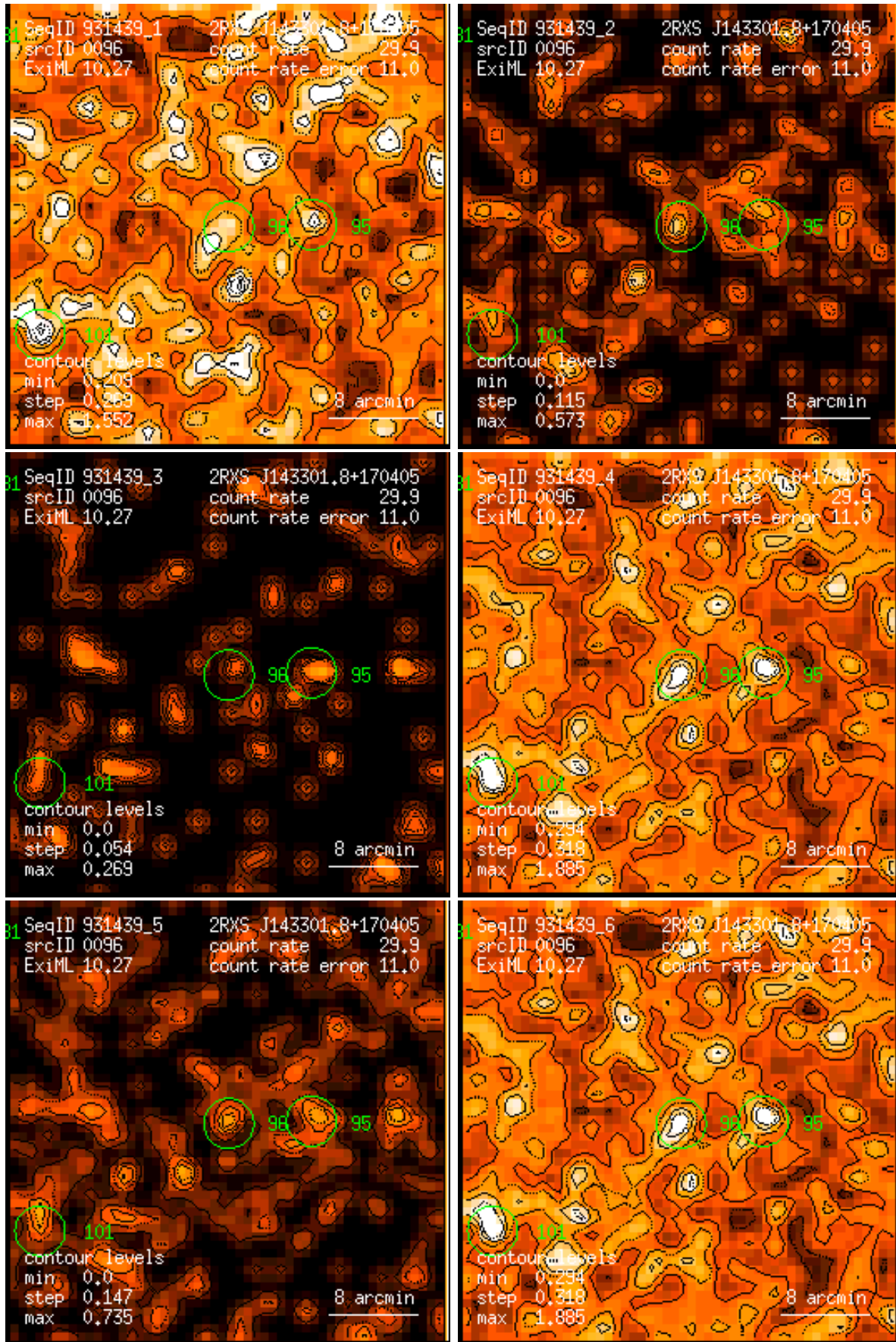
Figure 96: RASS 931439: detection 0096: band rate images, Gaussian filter: (1) PSPC channels 11 – 41, (2) 52 – 90, (3) 91 – 201, (4) 11 – 235, (5) 52 – 201, (6) 11 – 201. Broad band rates in counts/ks. Band rate contour levels in counts/ks/arcmin 2 .
