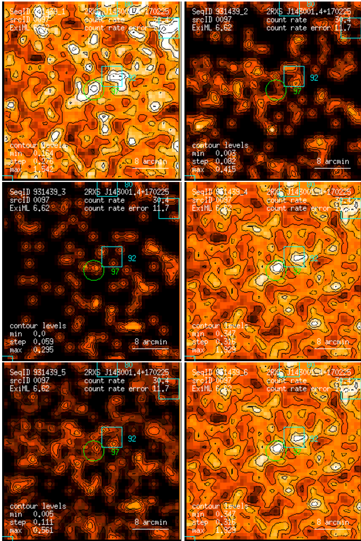
Figure 97: RASS 931439: detection 0097: band rate images, Gaussian filter: (1) PSPC channels 11 – 41, (2) 52 – 90, (3) 91 – 201, (4) 11 – 235, (5) 52 – 201, (6) 11 – 201. Broad band rates in counts/ks. Band rate contour levels in counts/ks/arcmin 2 .
