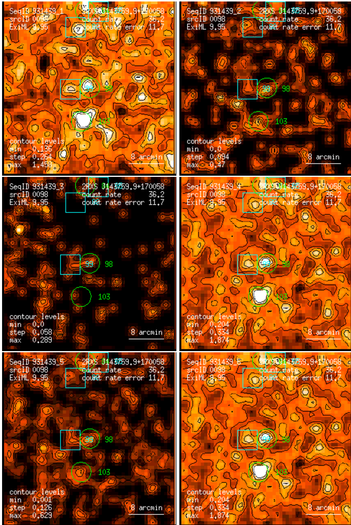
Figure 98: RASS 931439: detection 0098: band rate images, Gaussian filter: (1) PSPC channels 11 – 41, (2) 52 – 90, (3) 91 – 201, (4) 11 – 235, (5) 52 – 201, (6) 11 – 201. Broad band rates in counts/ks. Band rate contour levels in counts/ks/arcmin 2 .
