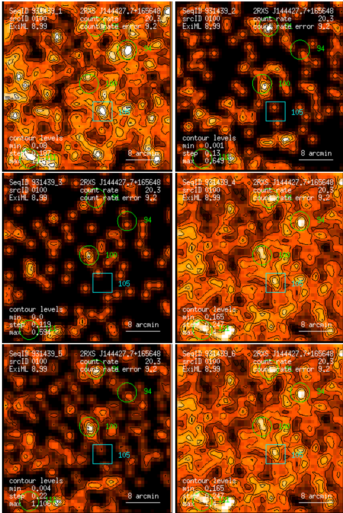
Figure 100: RASS 931439: detection 0100: band rate images, Gaussian filter: (1) PSPC channels 11 – 41, (2) 52 – 90, (3) 91 – 201, (4) 11 – 235, (5) 52 – 201, (6) 11 – 201. Broad band rates in counts/ks. Band rate contour levels in counts/ks/arcmin 2 .
