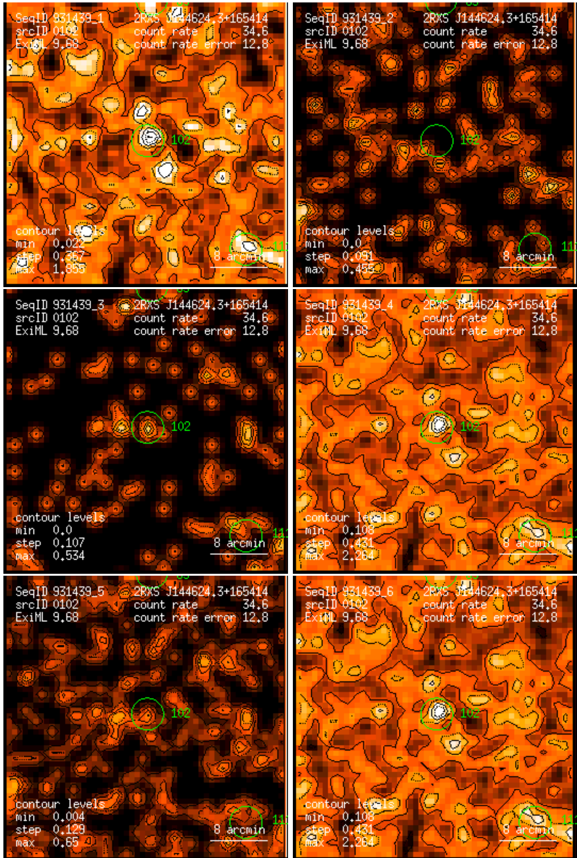
Figure 102: RASS 931439: detection 0102: band rate images, Gaussian filter: (1) PSPC channels 11 – 41, (2) 52 – 90, (3) 91 – 201, (4) 11 – 235, (5) 52 – 201, (6) 11 – 201. Broad band rates in counts/ks. Band rate contour levels in counts/ks/arcmin 2 .
