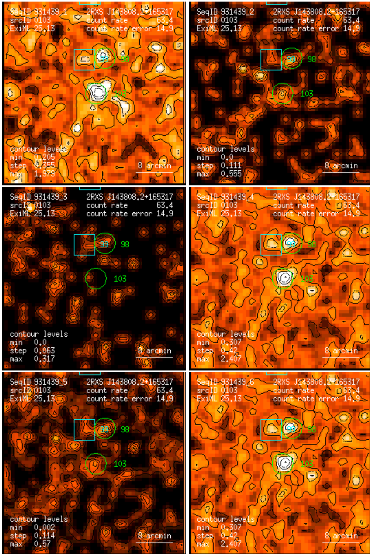
Figure 103: RASS 931439: detection 0103: band rate images, Gaussian filter: (1) PSPC channels 11 – 41, (2) 52 – 90, (3) 91 – 201, (4) 11 – 235, (5) 52 – 201, (6) 11 – 201. Broad band rates in counts/ks. Band rate contour levels in counts/ks/arcmin 2 .
