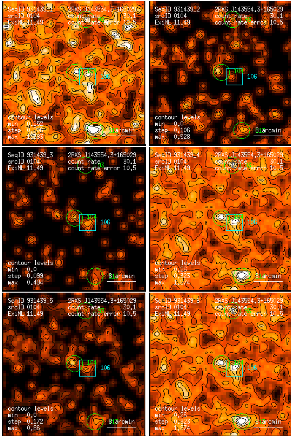
Figure 104: RASS 931439: detection 0104: band rate images, Gaussian filter: (1) PSPC channels 11 – 41, (2) 52 – 90, (3) 91 – 201, (4) 11 – 235, (5) 52 – 201, (6) 11 – 201. Broad band rates in counts/ks. Band rate contour levels in counts/ks/arcmin 2 .
