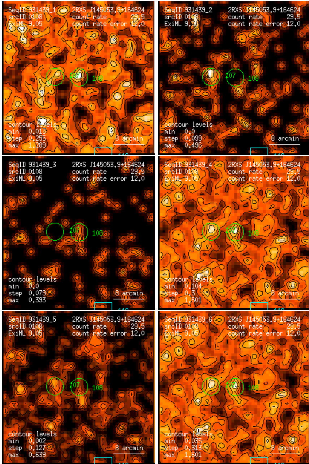
Figure 108: RASS 931439: detection 0108: band rate images, Gaussian filter: (1) PSPC channels 11 – 41, (2) 52 – 90, (3) 91 – 201, (4) 11 – 235, (5) 52 – 201, (6) 11 – 201. Broad band rates in counts/ks. Band rate contour levels in counts/ks/arcmin 2 .
