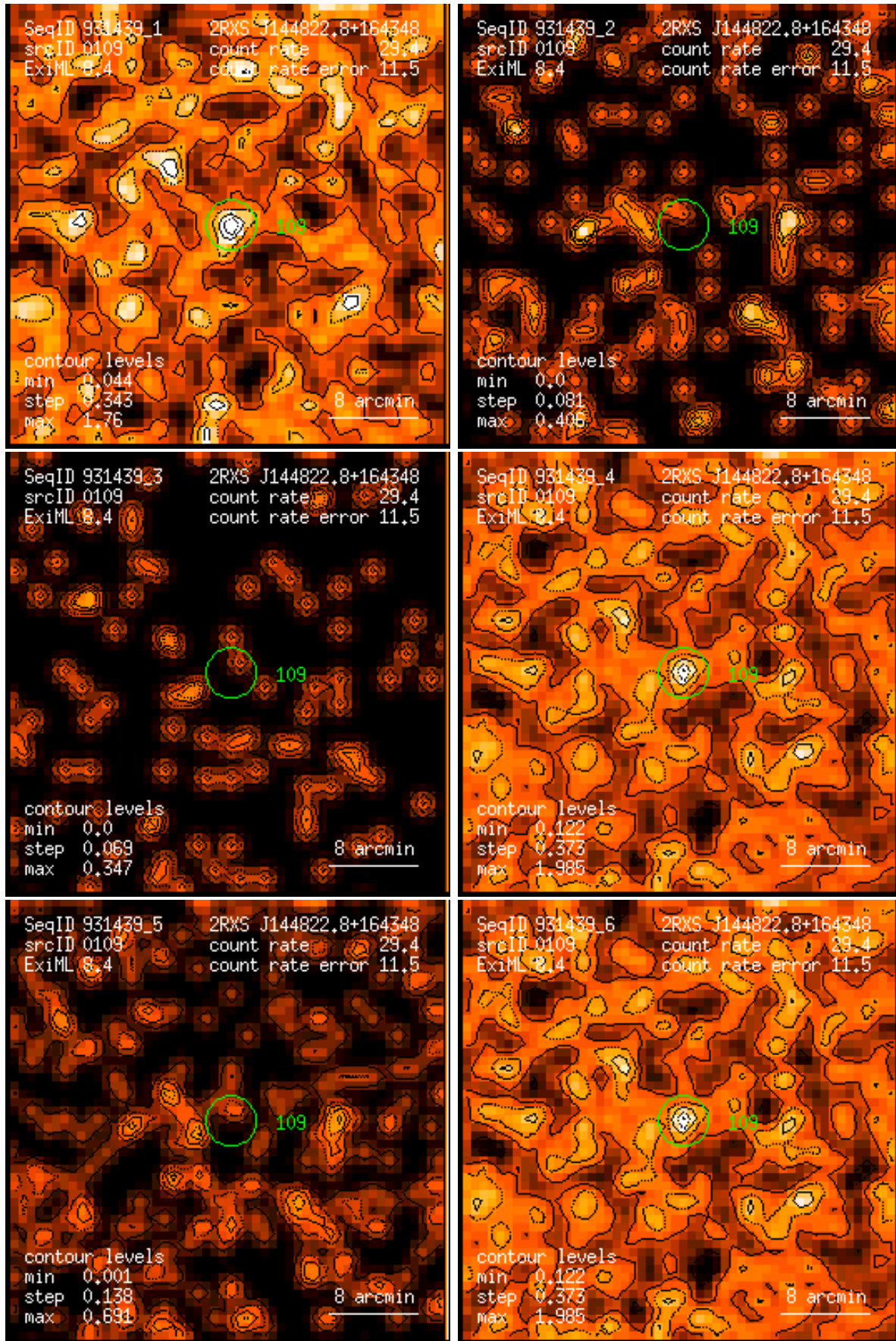
Figure 109: RASS 931439: detection 0109: band rate images, Gaussian filter: (1) PSPC channels 11 – 41, (2) 52 – 90, (3) 91 – 201, (4) 11 – 235, (5) 52 – 201, (6) 11 – 201. Broad band rates in counts/ks. Band rate contour levels in counts/ks/arcmin 2 .
