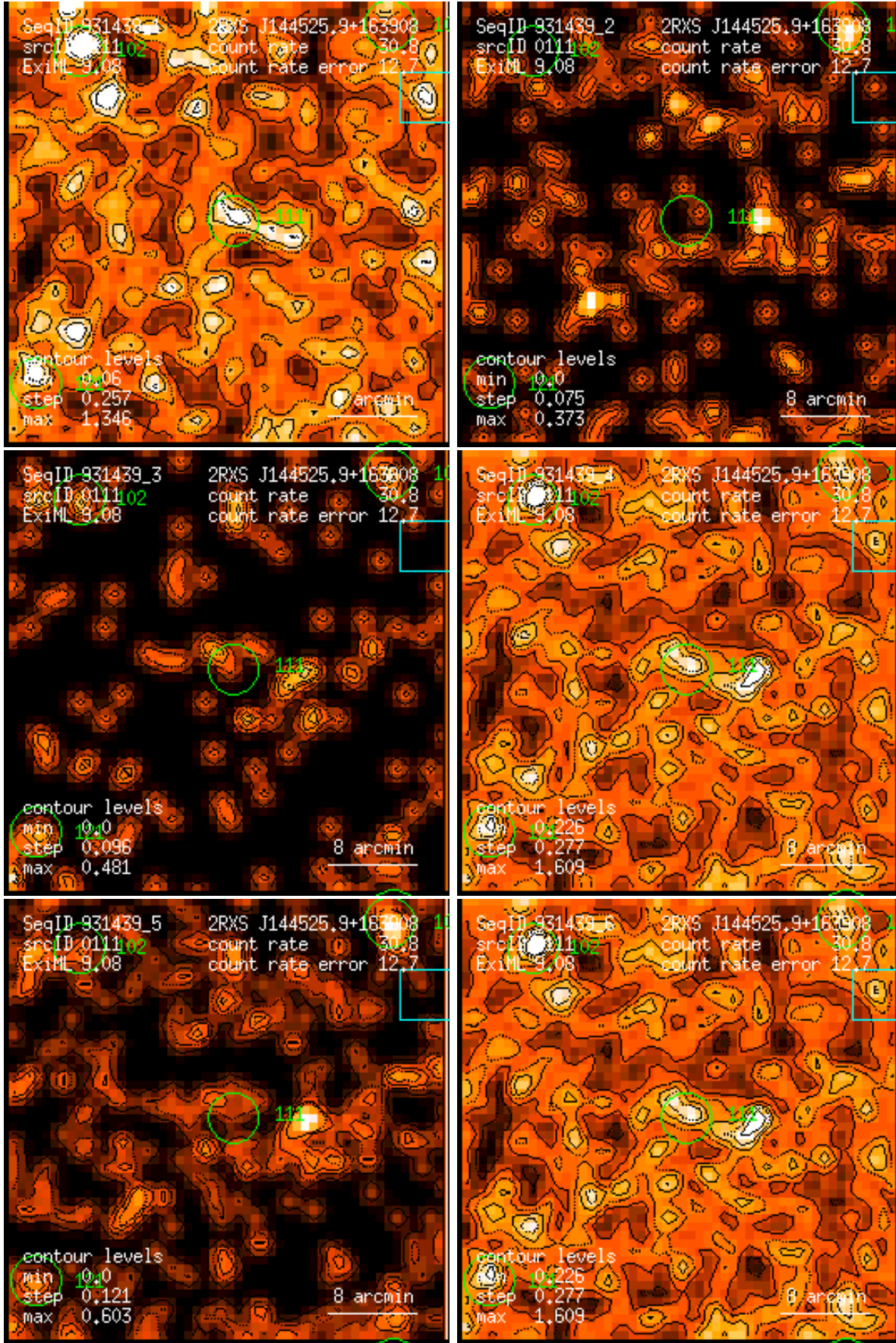
Figure 111: RASS 931439: detection 0111: band rate images, Gaussian filter: (1) PSPC channels 11 – 41, (2) 52 – 90, (3) 91 – 201, (4) 11 – 235, (5) 52 – 201, (6) 11 – 201. Broad band rates in counts/ks. Band rate contour levels in counts/ks/arcmin 2 .
