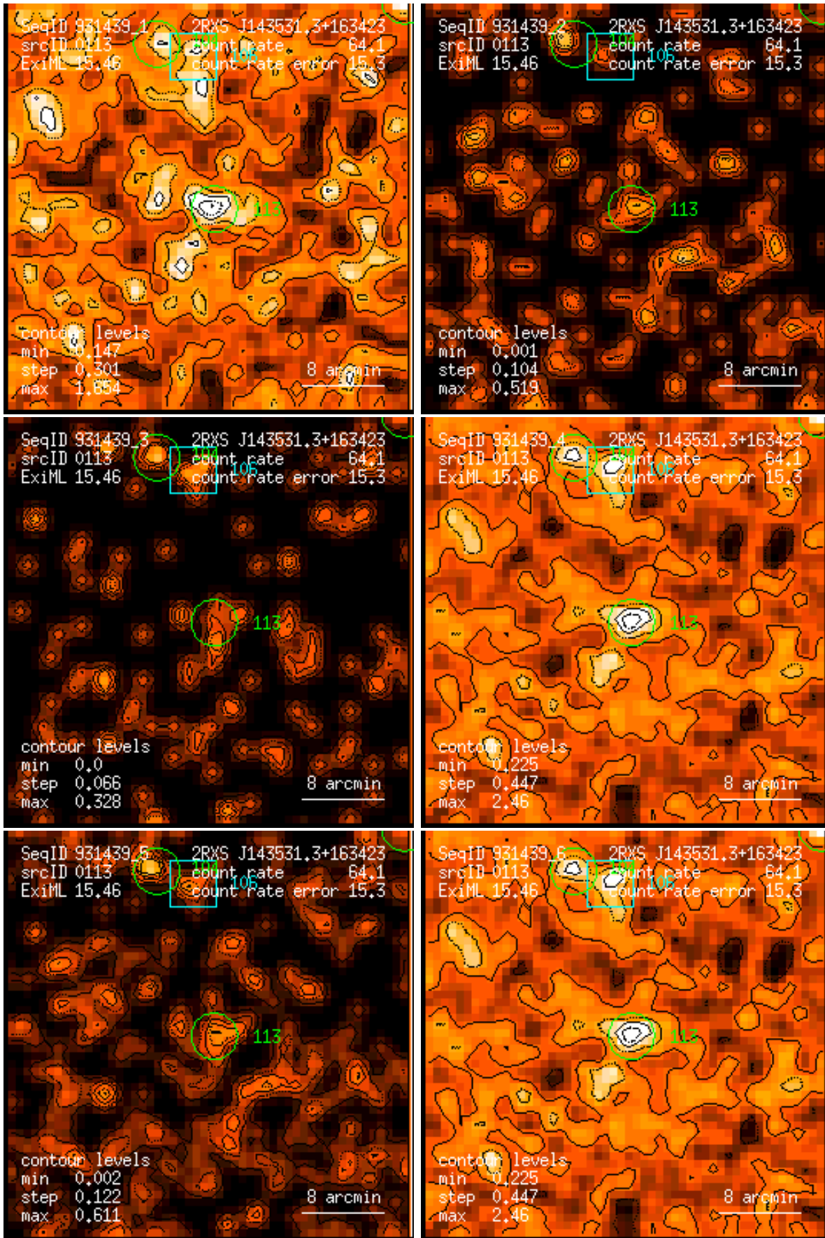
Figure 113: RASS 931439: detection 0113: band rate images, Gaussian filter: (1) PSPC channels 11 – 41, (2) 52 – 90, (3) 91 – 201, (4) 11 – 235, (5) 52 – 201, (6) 11 – 201. Broad band rates in counts/ks. Band rate contour levels in counts/ks/arcmin 2 .
