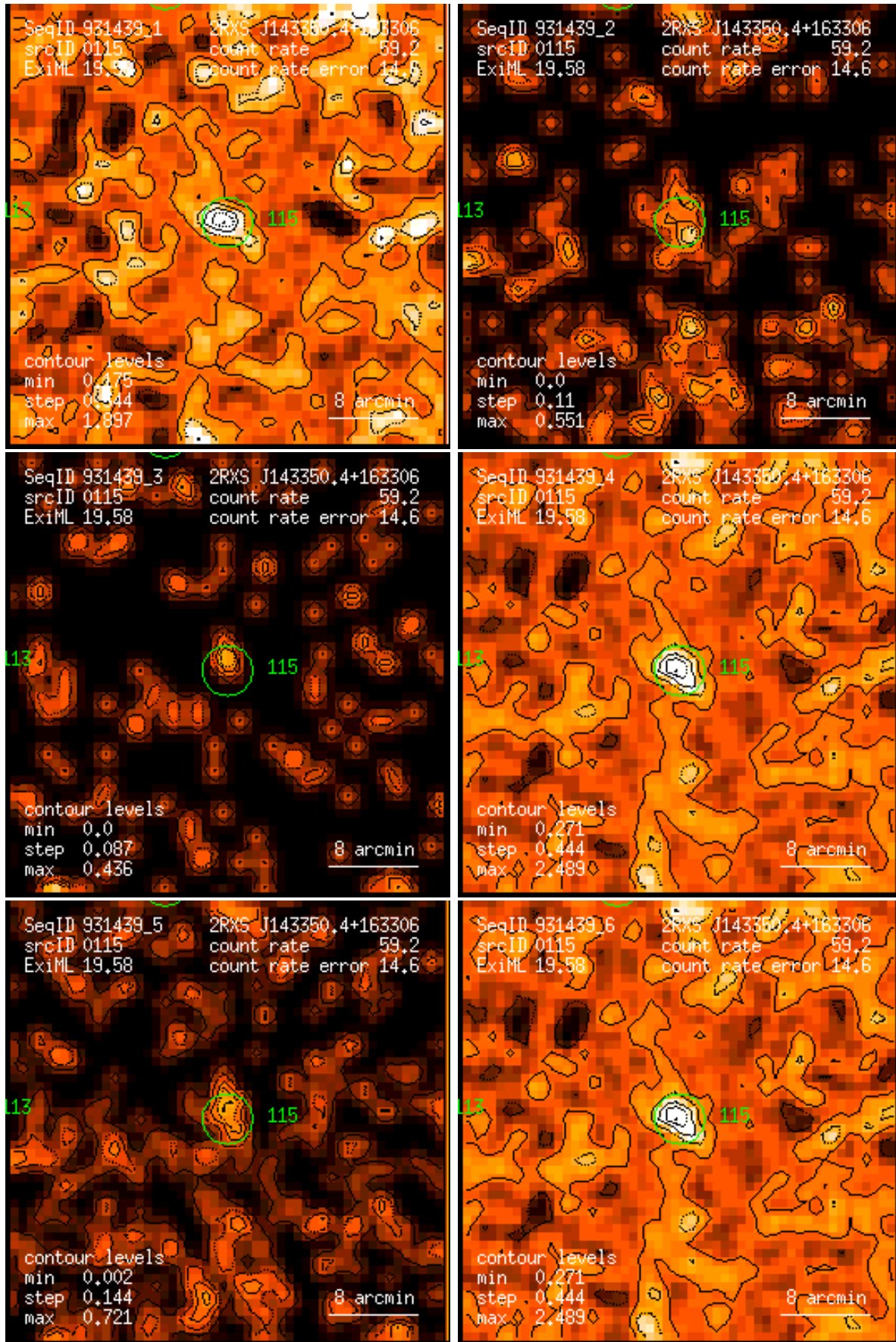
Figure 115: RASS 931439: detection 0115: band rate images, Gaussian filter: (1) PSPC channels 11 – 41, (2) 52 – 90, (3) 91 – 201, (4) 11 – 235, (5) 52 – 201, (6) 11 – 201. Broad band rates in counts/ks. Band rate contour levels in counts/ks/arcmin 2 .
