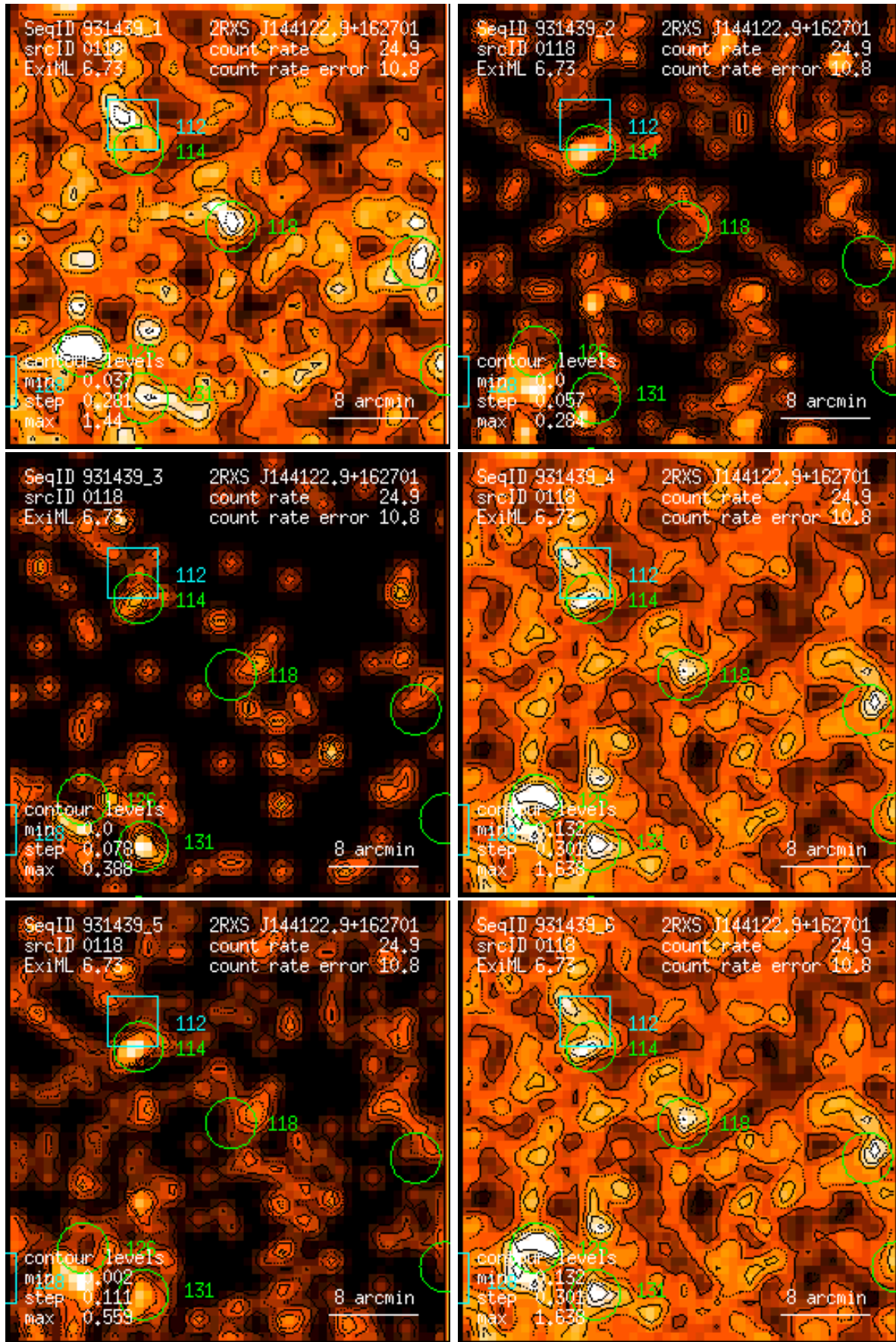
Figure 118: RASS 931439: detection 0118: band rate images, Gaussian filter: (1) PSPC channels 11 – 41, (2) 52 – 90, (3) 91 – 201, (4) 11 – 235, (5) 52 – 201, (6) 11 – 201. Broad band rates in counts/ks. Band rate contour levels in counts/ks/arcmin 2 .
