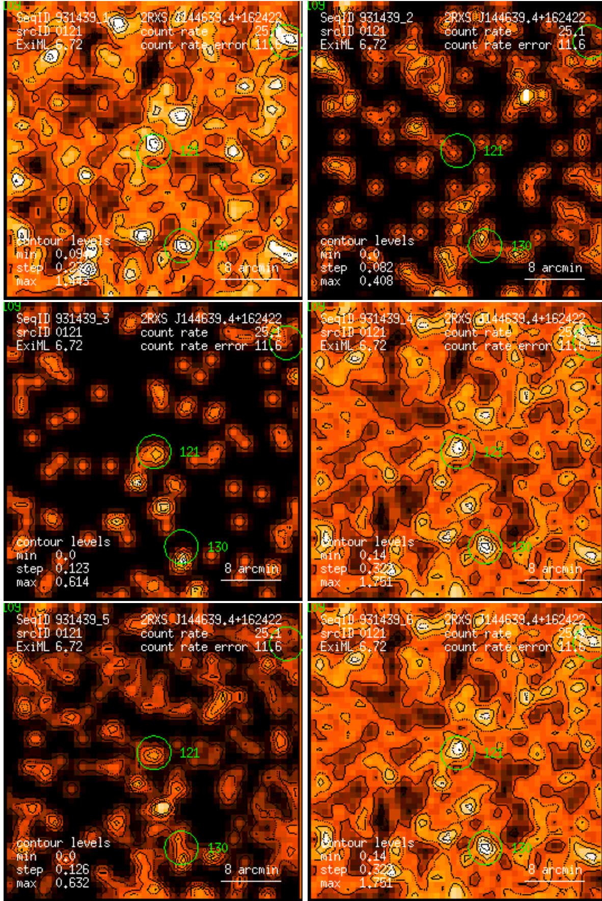
Figure 121: RASS 931439: detection 0121: band rate images, Gaussian filter: (1) PSPC channels 11 – 41, (2) 52 – 90, (3) 91 – 201, (4) 11 – 235, (5) 52 – 201, (6) 11 – 201. Broad band rates in counts/ks. Band rate contour levels in counts/ks/arcmin 2 .
