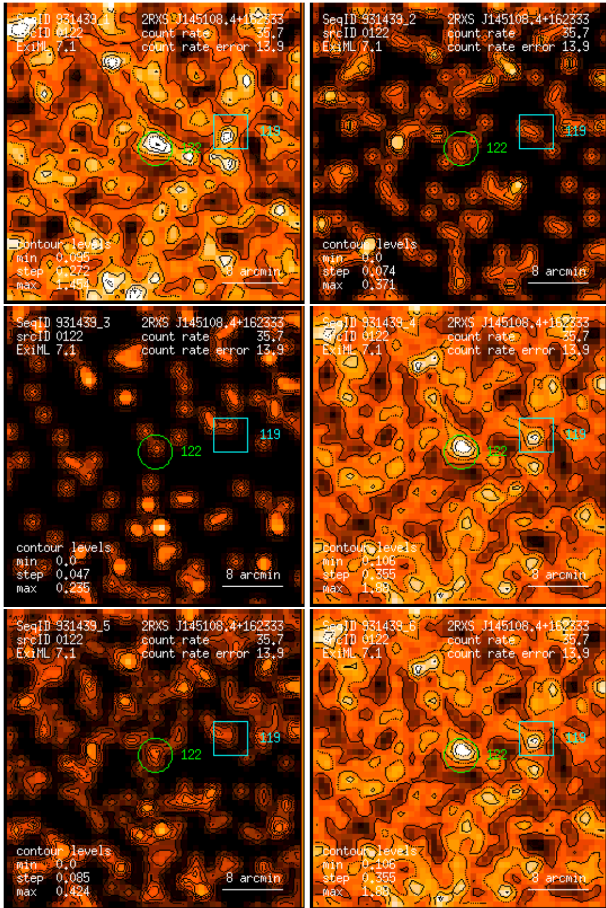
Figure 122: RASS 931439: detection 0122: band rate images, Gaussian filter: (1) PSPC channels 11 – 41, (2) 52 – 90, (3) 91 – 201, (4) 11 – 235, (5) 52 – 201, (6) 11 – 201. Broad band rates in counts/ks. Band rate contour levels in counts/ks/arcmin 2 .
