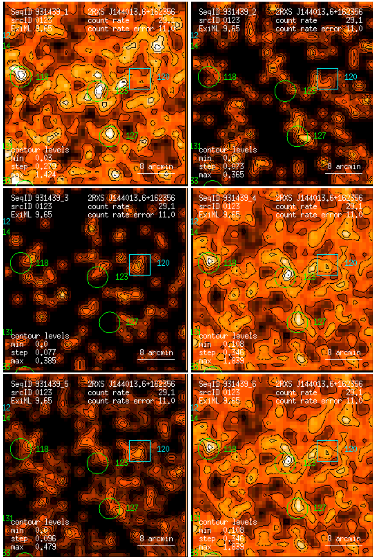
Figure 123: RASS 931439: detection 0123: band rate images, Gaussian filter: (1) PSPC channels 11 – 41, (2) 52 – 90, (3) 91 – 201, (4) 11 – 235, (5) 52 – 201, (6) 11 – 201. Broad band rates in counts/ks. Band rate contour levels in counts/ks/arcmin 2 .
