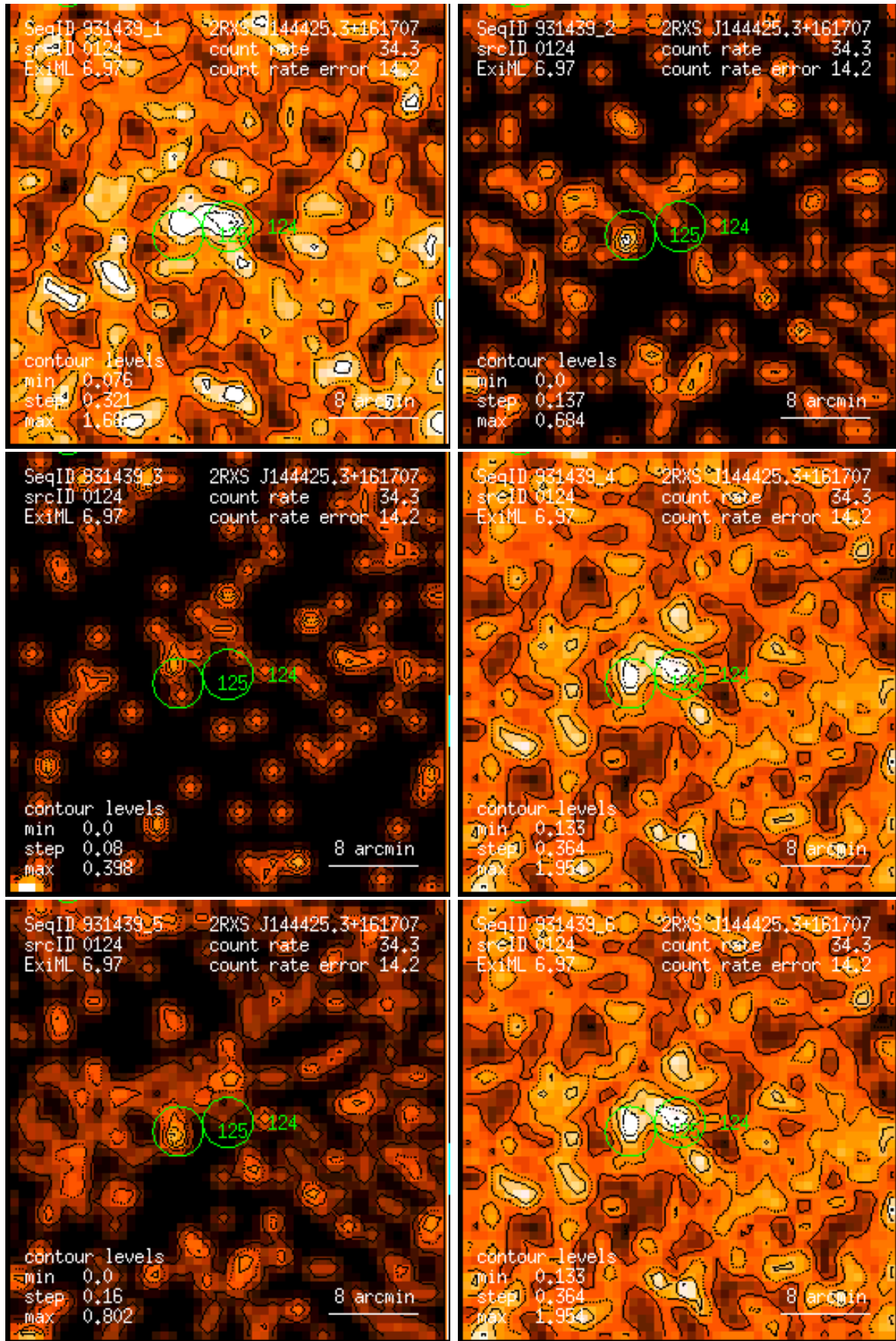
Figure 124: RASS 931439: detection 0124: band rate images, Gaussian filter: (1) PSPC channels 11 – 41, (2) 52 – 90, (3) 91 – 201, (4) 11 – 235, (5) 52 – 201, (6) 11 – 201. Broad band rates in counts/ks. Band rate contour levels in counts/ks/arcmin 2 .
