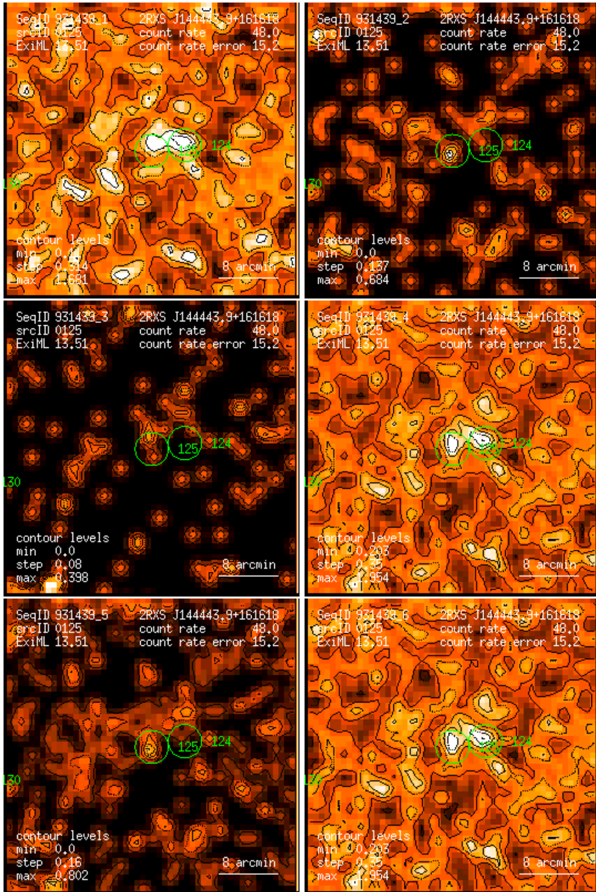
Figure 125: RASS 931439: detection 0125: band rate images, Gaussian filter: (1) PSPC channels 11 – 41, (2) 52 – 90, (3) 91 – 201, (4) 11 – 235, (5) 52 – 201, (6) 11 – 201. Broad band rates in counts/ks. Band rate contour levels in counts/ks/arcmin 2 .
