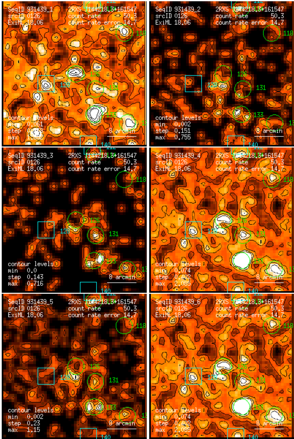
Figure 126: RASS 931439: detection 0126: band rate images, Gaussian filter: (1) PSPC channels 11 – 41, (2) 52 – 90, (3) 91 – 201, (4) 11 – 235, (5) 52 – 201, (6) 11 – 201. Broad band rates in counts/ks. Band rate contour levels in counts/ks/arcmin 2 .
