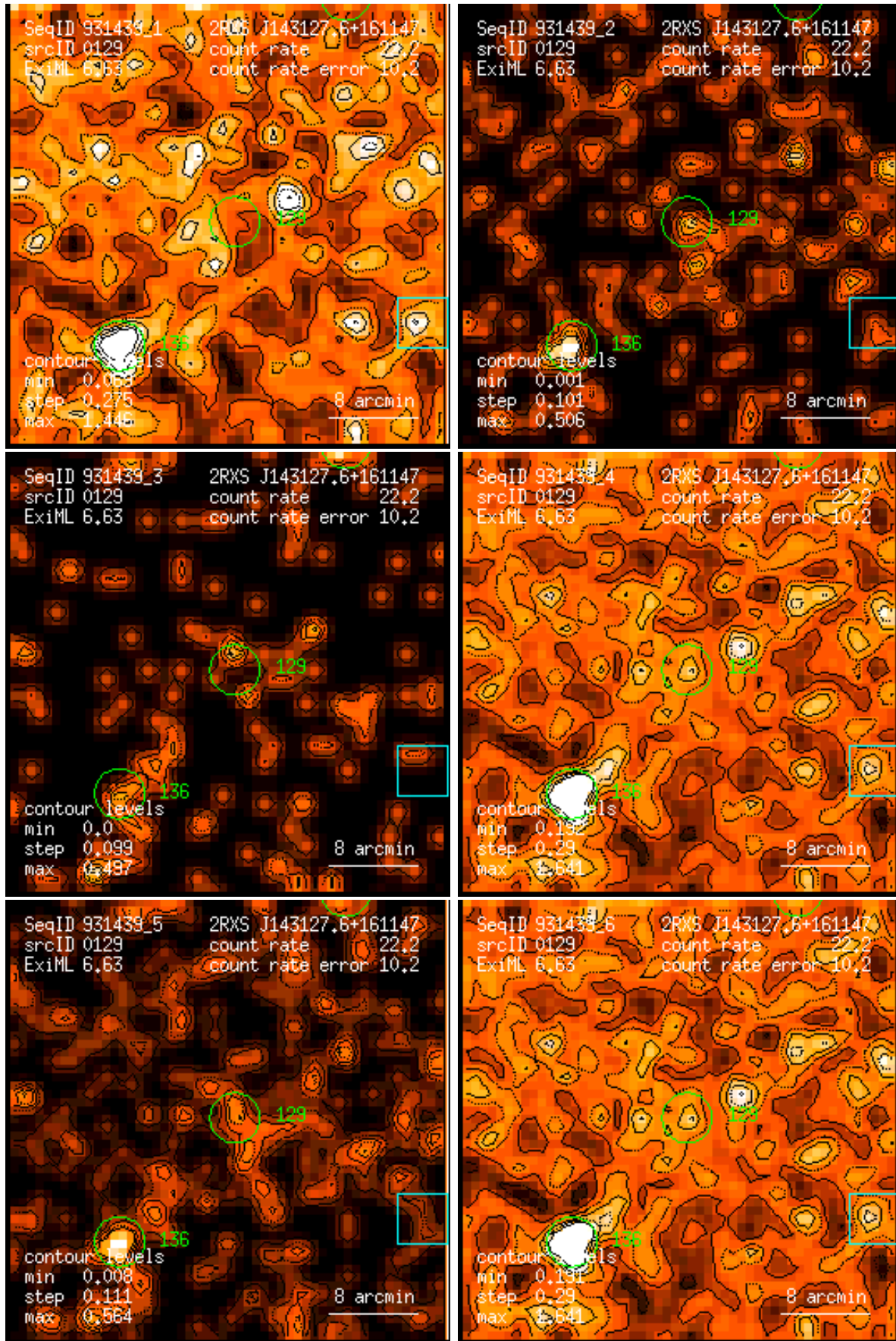
Figure 129: RASS 931439: detection 0129: band rate images, Gaussian filter: (1) PSPC channels 11 – 41, (2) 52 – 90, (3) 91 – 201, (4) 11 – 235, (5) 52 – 201, (6) 11 – 201. Broad band rates in counts/ks. Band rate contour levels in counts/ks/arcmin 2 .
