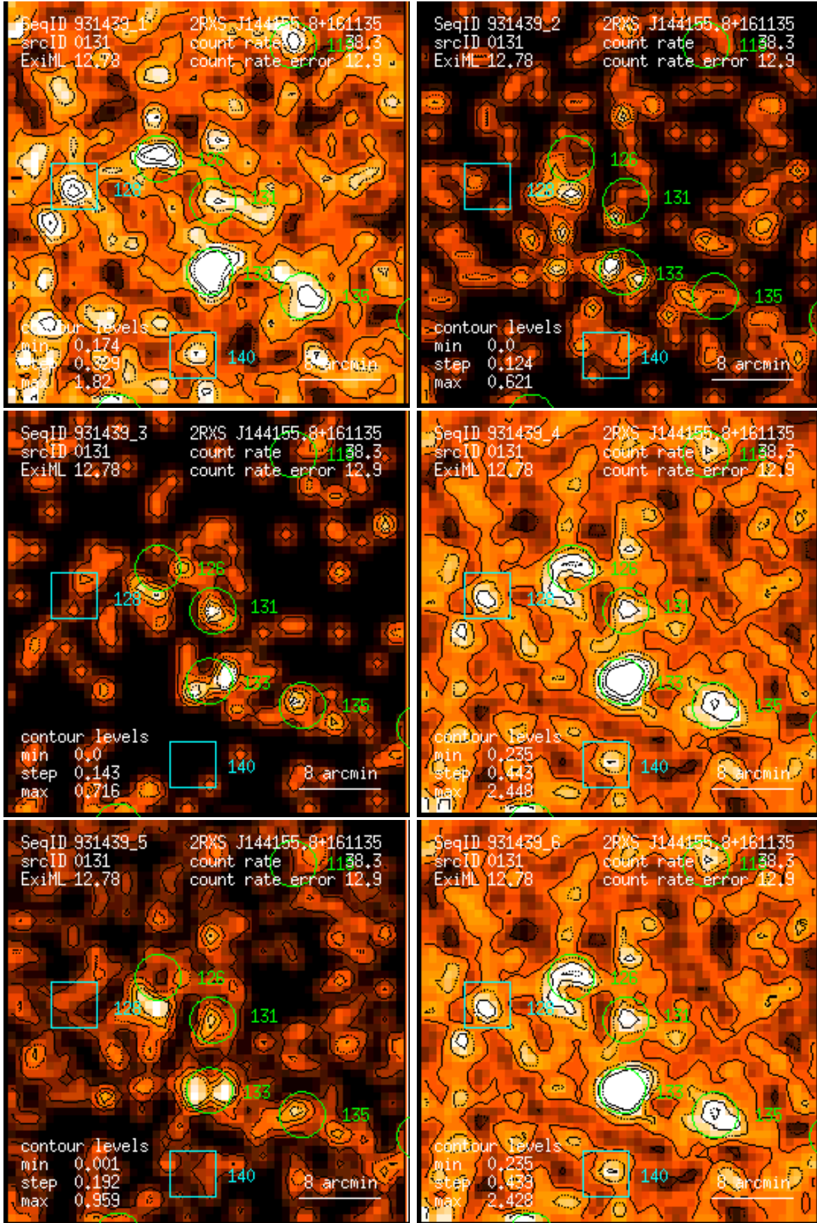
Figure 131: RASS 931439: detection 0131: band rate images, Gaussian filter: (1) PSPC channels 11 – 41, (2) 52 – 90, (3) 91 – 201, (4) 11 – 235, (5) 52 – 201, (6) 11 – 201. Broad band rates in counts/ks. Band rate contour levels in counts/ks/arcmin 2 .
