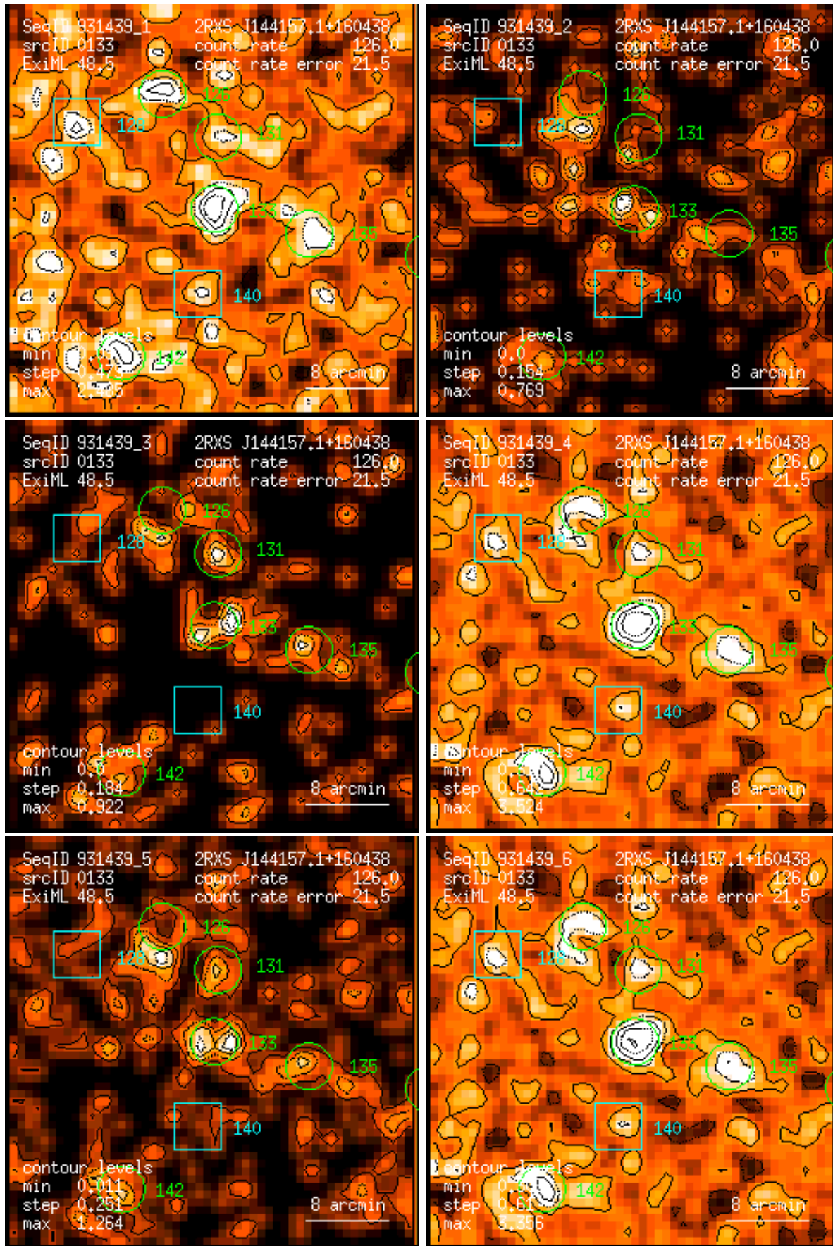
Figure 133: RASS 931439: detection 0133: band rate images, Gaussian filter: (1) PSPC channels 11 – 41, (2) 52 – 90, (3) 91 – 201, (4) 11 – 235, (5) 52 – 201, (6) 11 – 201. Broad band rates in counts/ks. Band rate contour levels in counts/ks/arcmin 2 .
