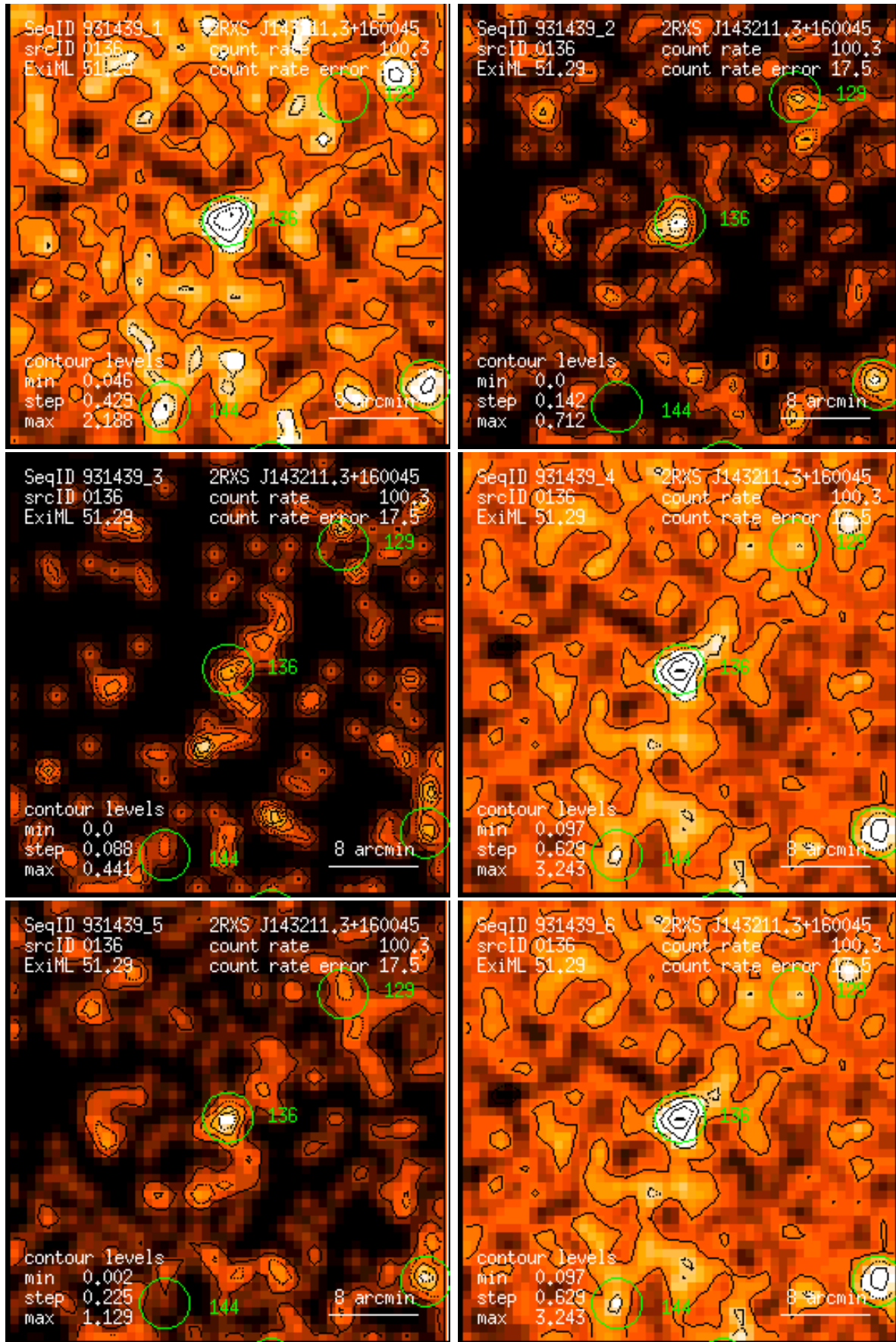
Figure 136: RASS 931439: detection 0136: band rate images, Gaussian filter: (1) PSPC channels 11 – 41, (2) 52 – 90, (3) 91 – 201, (4) 11 – 235, (5) 52 – 201, (6) 11 – 201. Broad band rates in counts/ks. Band rate contour levels in counts/ks/arcmin 2 .
