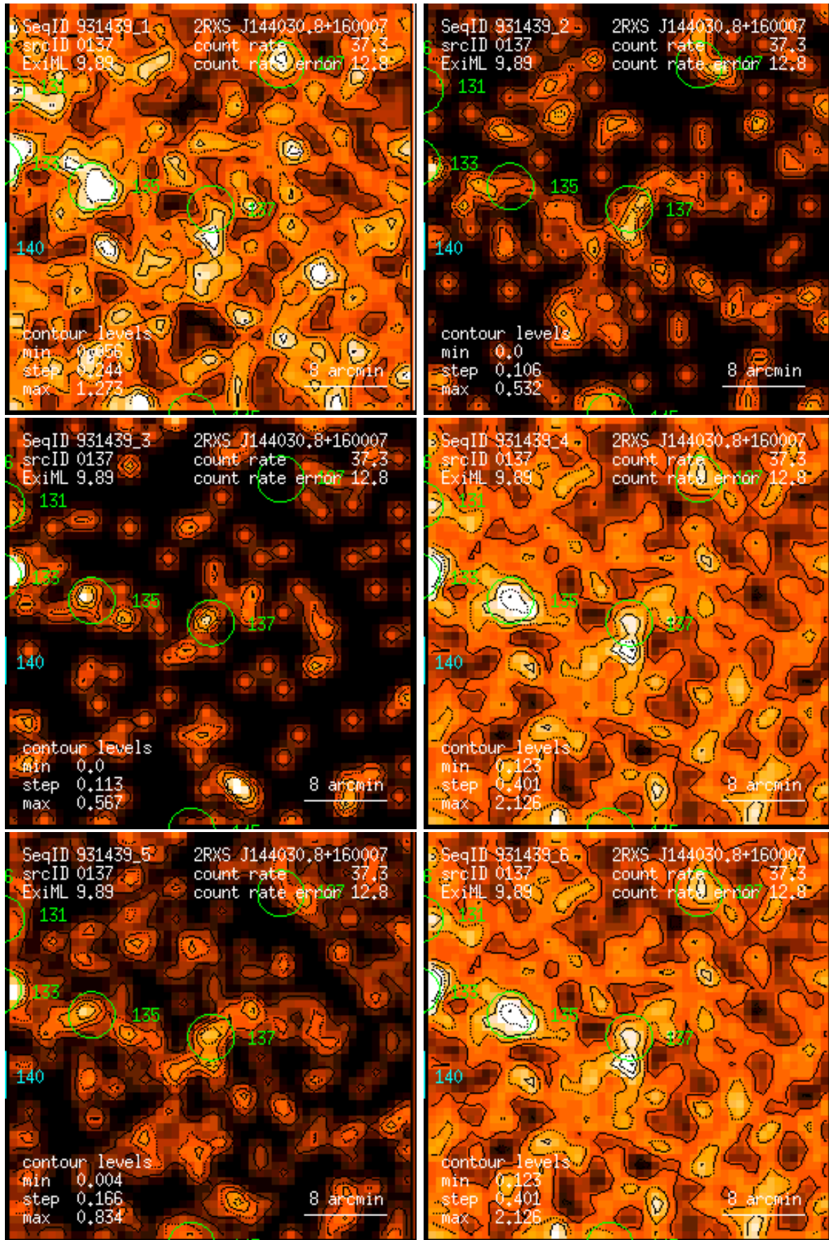
Figure 137: RASS 931439: detection 0137: band rate images, Gaussian filter: (1) PSPC channels 11 – 41, (2) 52 – 90, (3) 91 – 201, (4) 11 – 235, (5) 52 – 201, (6) 11 – 201. Broad band rates in counts/ks. Band rate contour levels in counts/ks/arcmin 2 .
