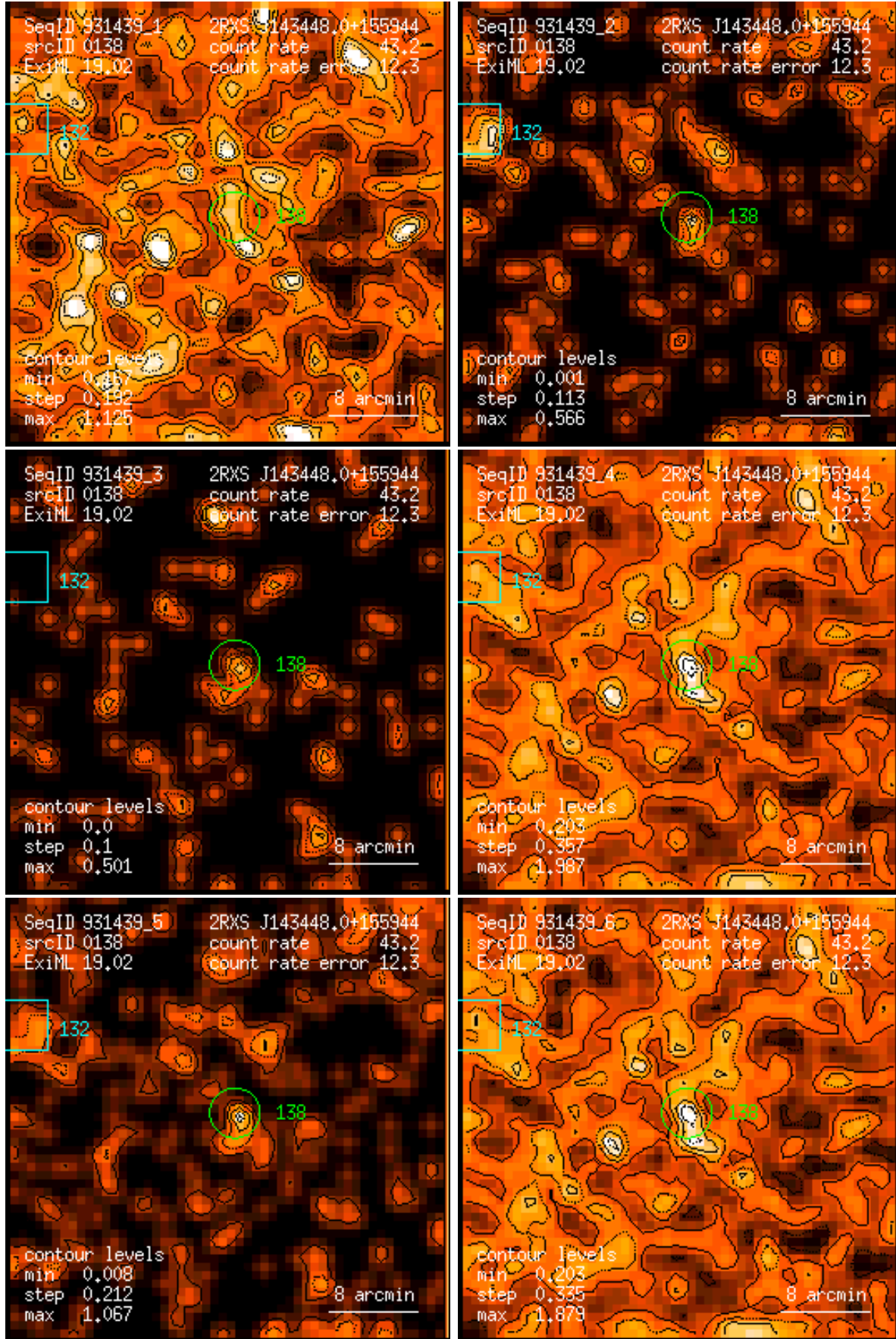
Figure 138: RASS 931439: detection 0138: band rate images, Gaussian filter: (1) PSPC channels 11 – 41, (2) 52 – 90, (3) 91 – 201, (4) 11 – 235, (5) 52 – 201, (6) 11 – 201. Broad band rates in counts/ks. Band rate contour levels in counts/ks/arcmin 2 .
