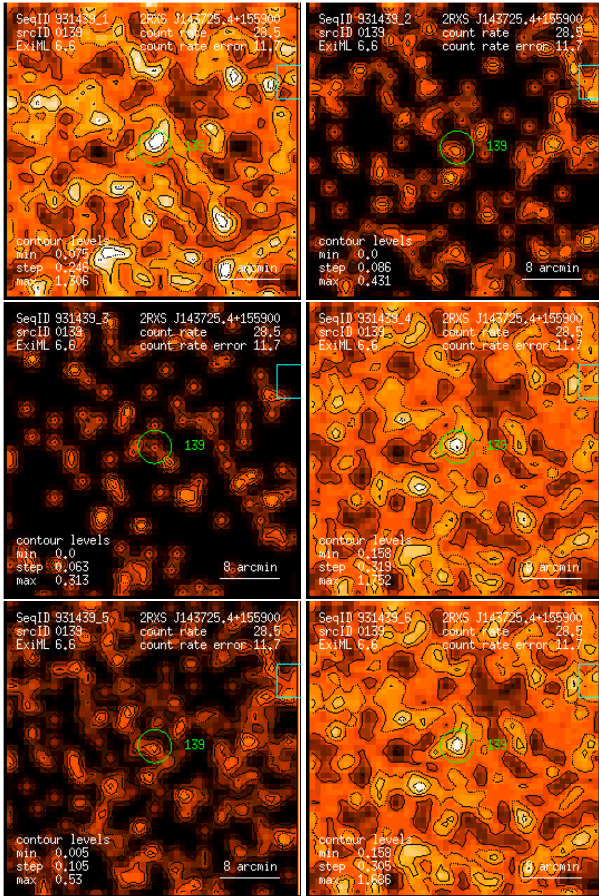
Figure 139: RASS 931439: detection 0139: band rate images, Gaussian filter: (1) PSPC channels 11 – 41, (2) 52 – 90, (3) 91 – 201, (4) 11 – 235, (5) 52 – 201, (6) 11 – 201. Broad band rates in counts/ks. Band rate contour levels in counts/ks/arcmin 2 .
