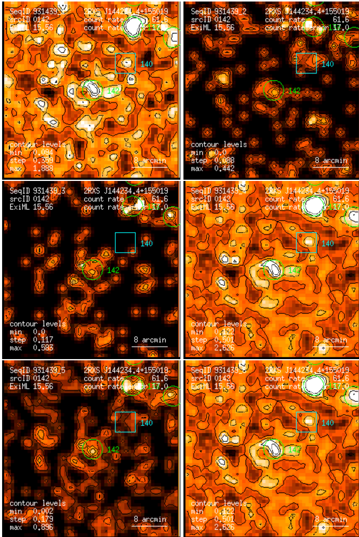
Figure 142: RASS 931439: detection 0142: band rate images, Gaussian filter: (1) PSPC channels 11 – 41, (2) 52 – 90, (3) 91 – 201, (4) 11 – 235, (5) 52 – 201, (6) 11 – 201. Broad band rates in counts/ks. Band rate contour levels in counts/ks/arcmin 2 .
