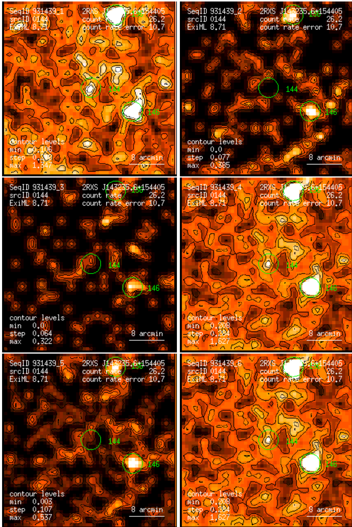
Figure 144: RASS 931439: detection 0144: band rate images, Gaussian filter: (1) PSPC channels 11 – 41, (2) 52 – 90, (3) 91 – 201, (4) 11 – 235, (5) 52 – 201, (6) 11 – 201. Broad band rates in counts/ks. Band rate contour levels in counts/ks/arcmin 2 .
