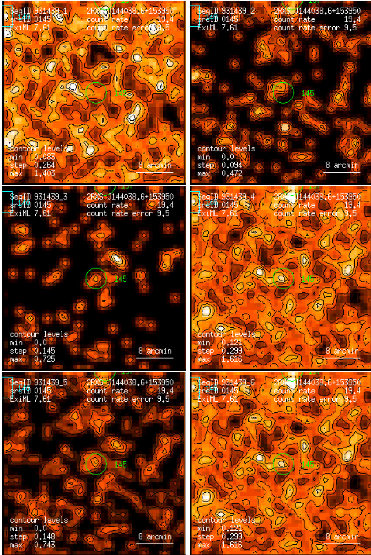
Figure 145: RASS 931439: detection 0145: band rate images, Gaussian filter: (1) PSPC channels 11 – 41, (2) 52 – 90, (3) 91 – 201, (4) 11 – 235, (5) 52 – 201, (6) 11 – 201. Broad band rates in counts/ks. Band rate contour levels in counts/ks/arcmin 2 .
